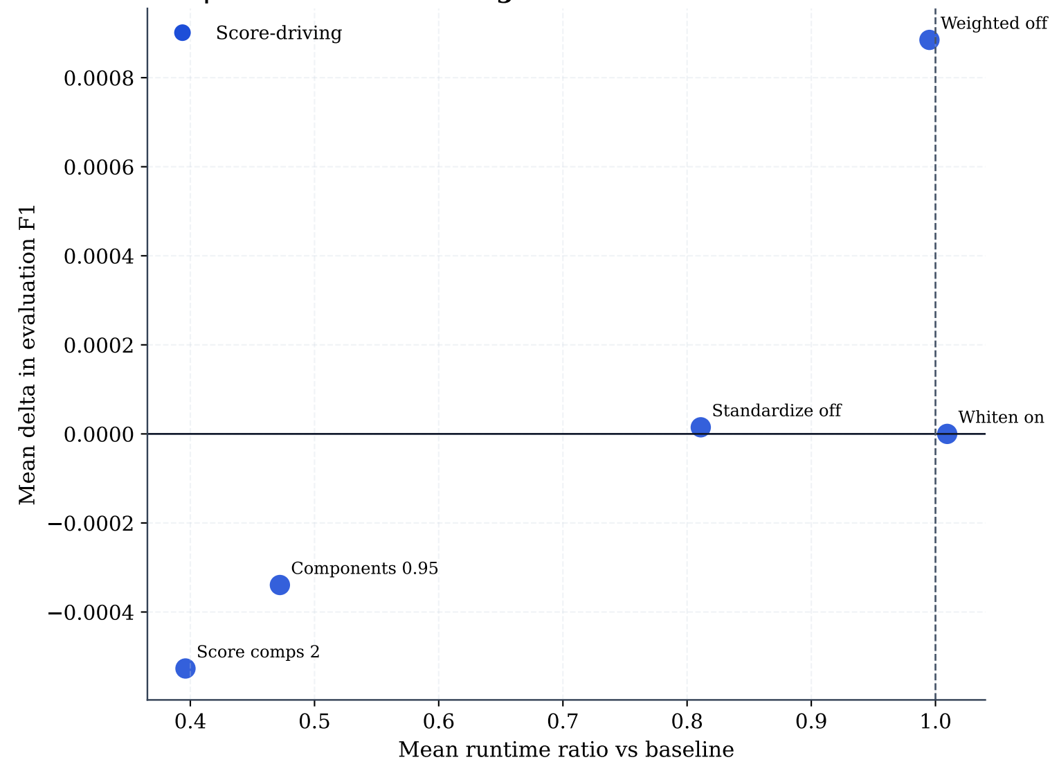
PCA | Runtime tradeoff against mean delta in evaluation F1
