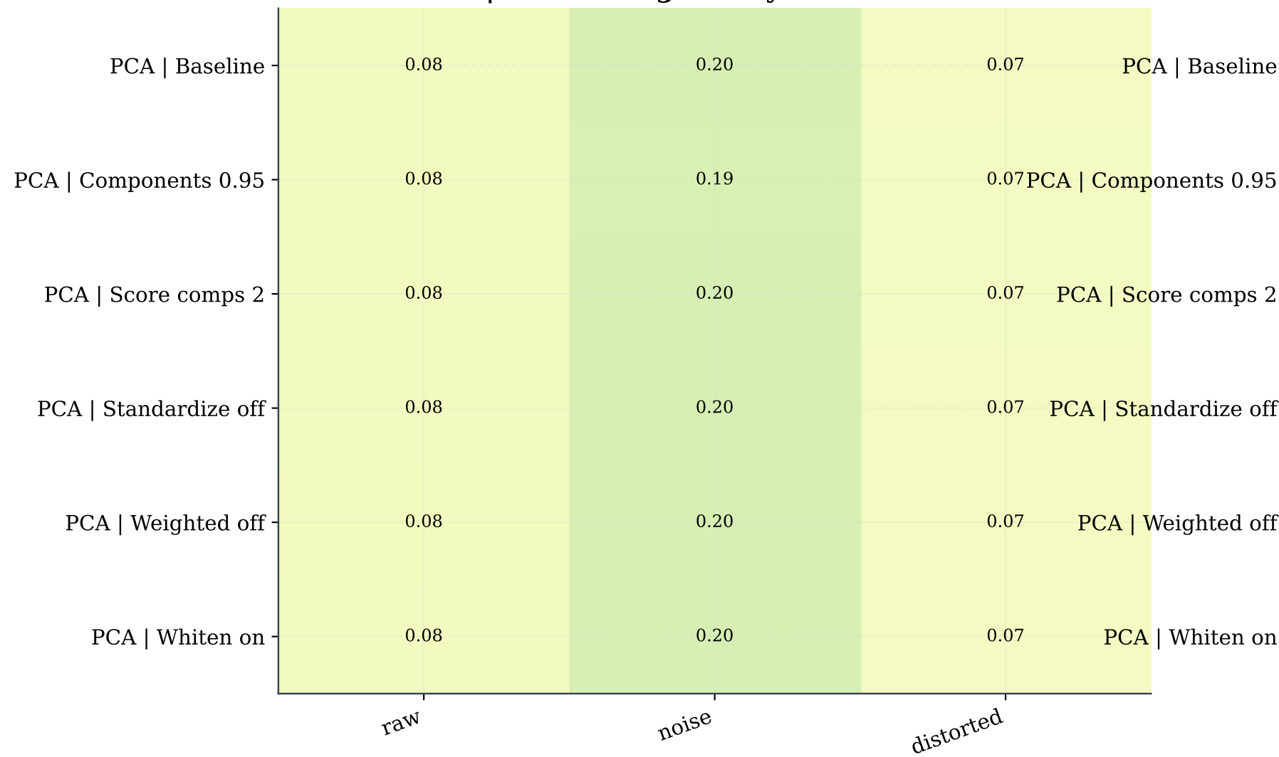
PCA | Mean Range F1 by dataset variant
