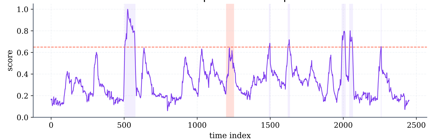
Variant 6: Standardize off | Eval F1=0.00 | ROC AUC=0.92
