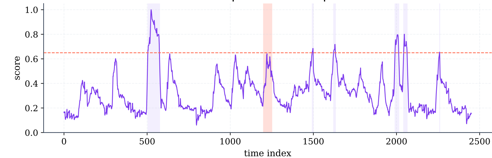
Variant 3: Score comps 2 | Eval F1=0.00 | ROC AUC=0.92
