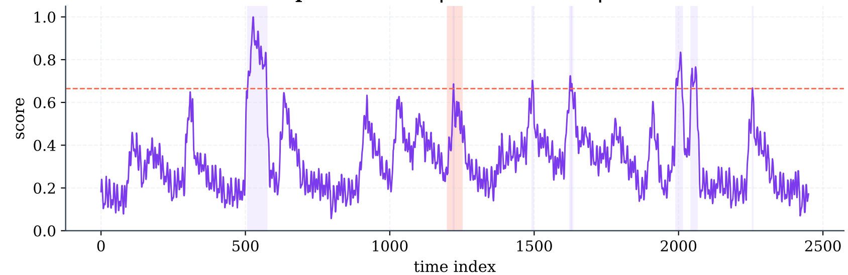
Variant 4: Whiten on | Eval F1=0.00 | ROC AUC=0.92
