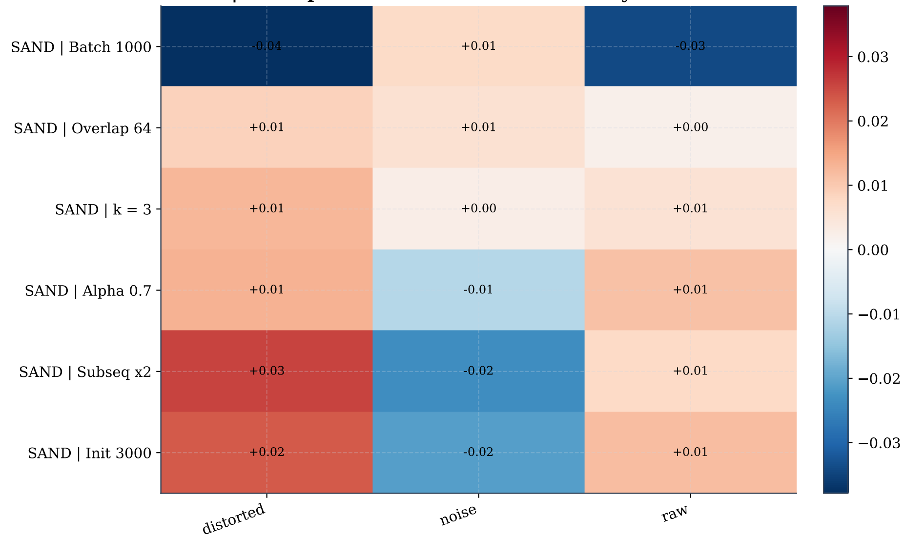
SAND | Mean paired delta in evaluation F1 by dataset variant
