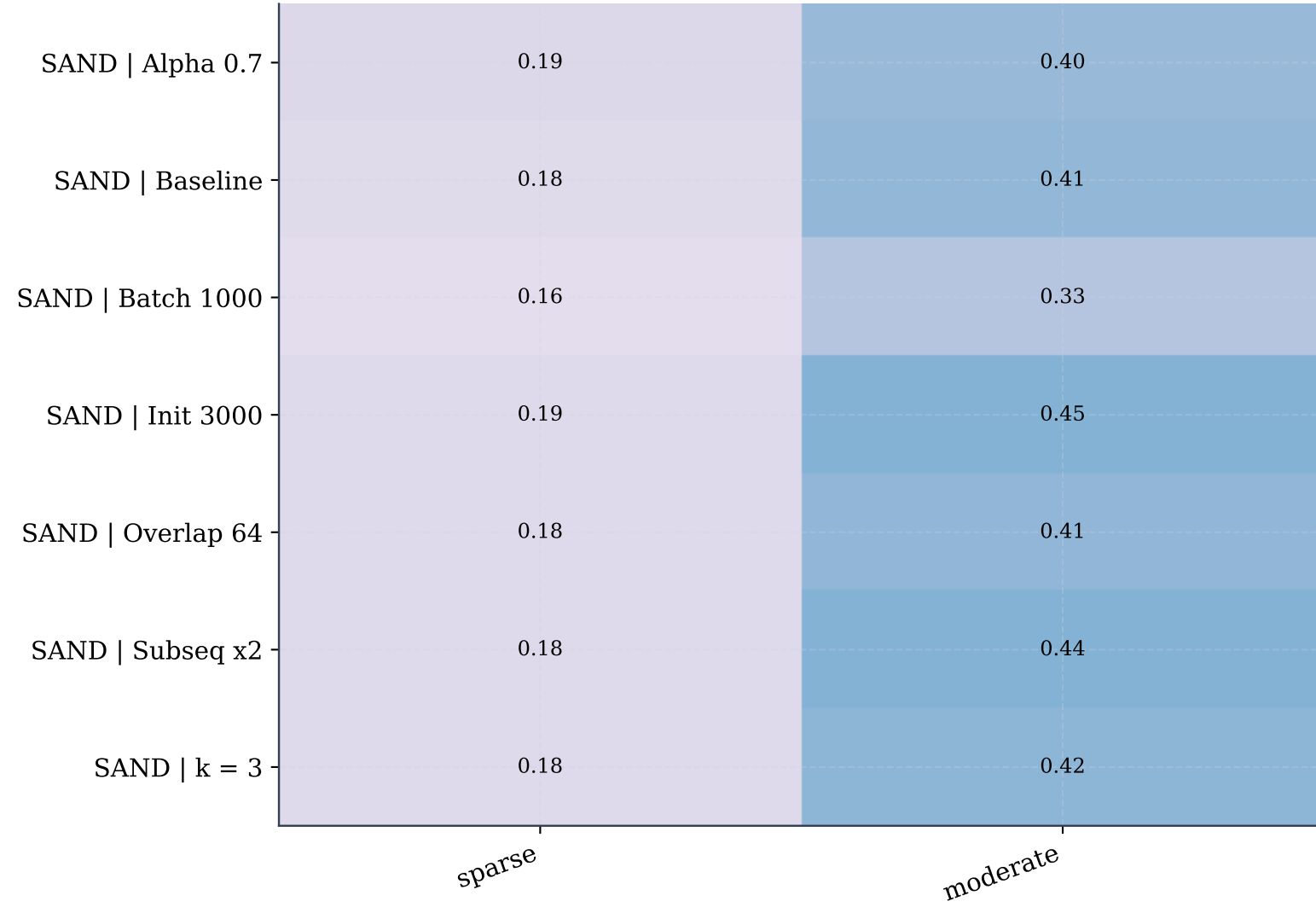
SAND | Mean Range F1 by anomaly ratio
