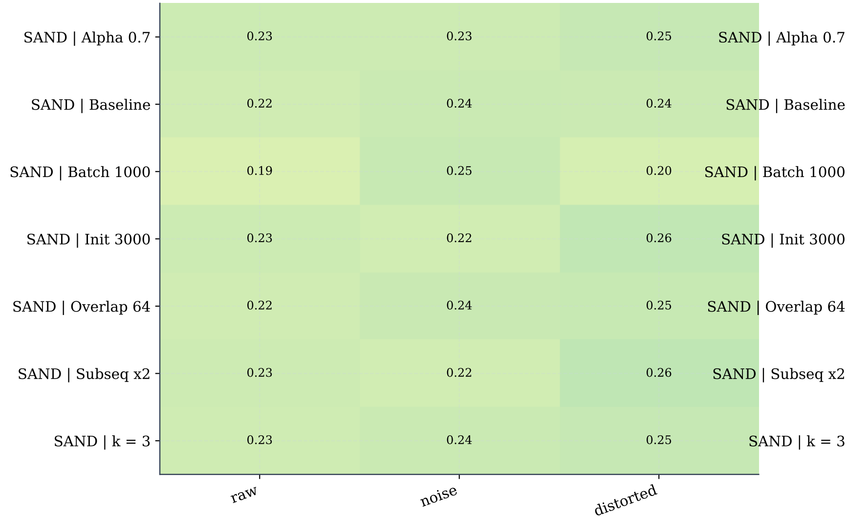
SAND | Mean Range F1 by dataset variant
