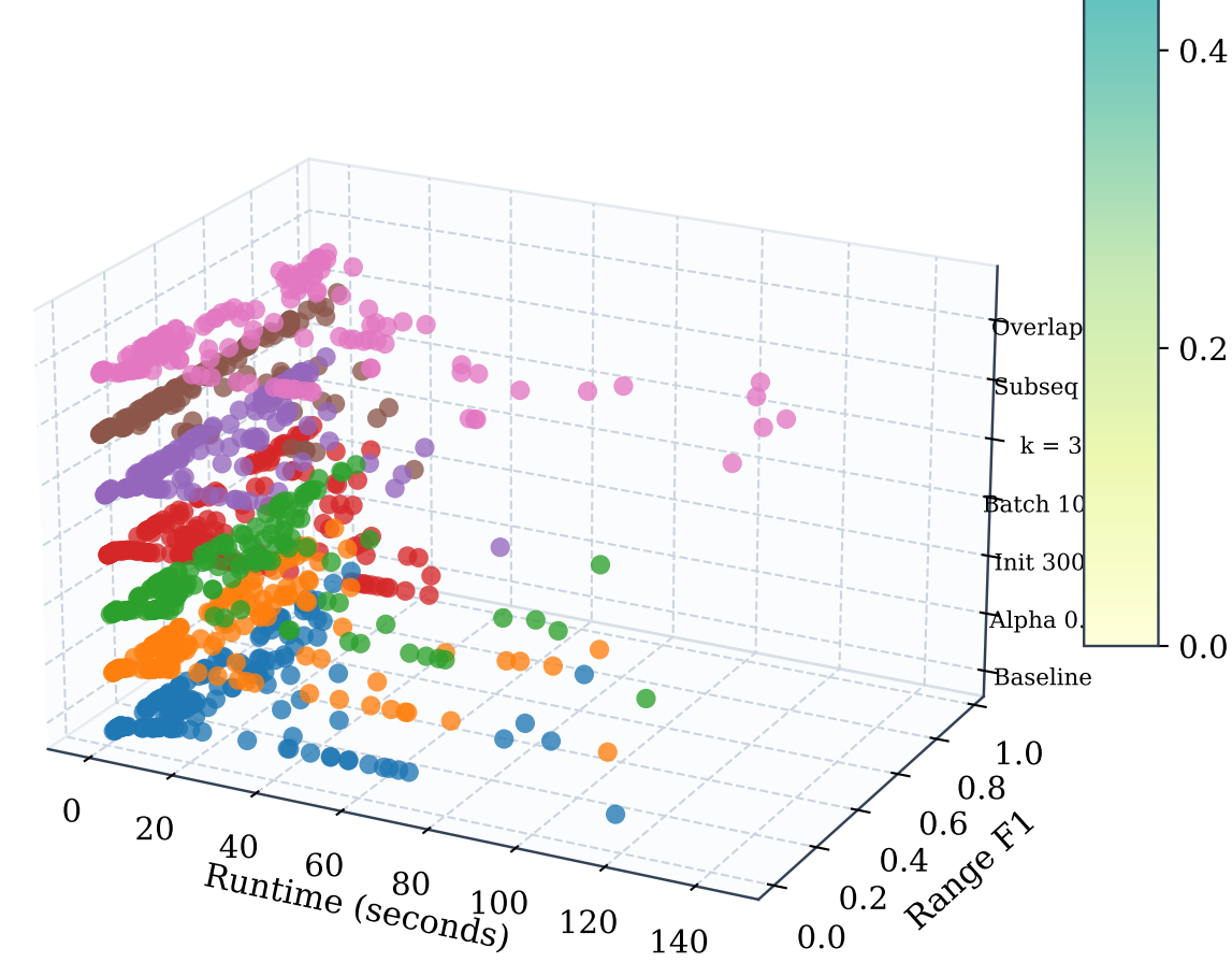
SAND | Layered 3D runtime vs Range F1
