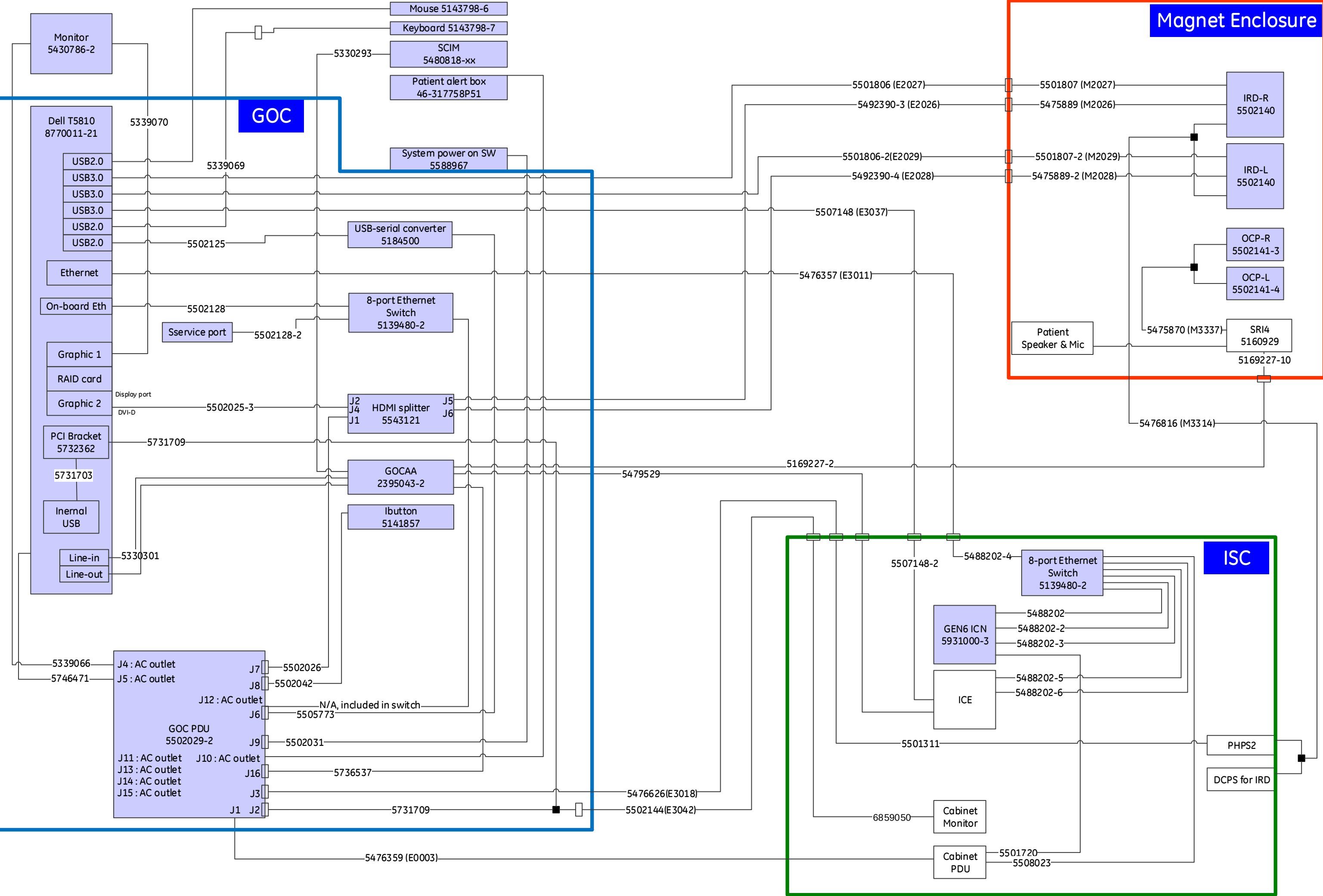
KIZUNA1.5T OW&ICN&IRD&OCP Block Diagram
