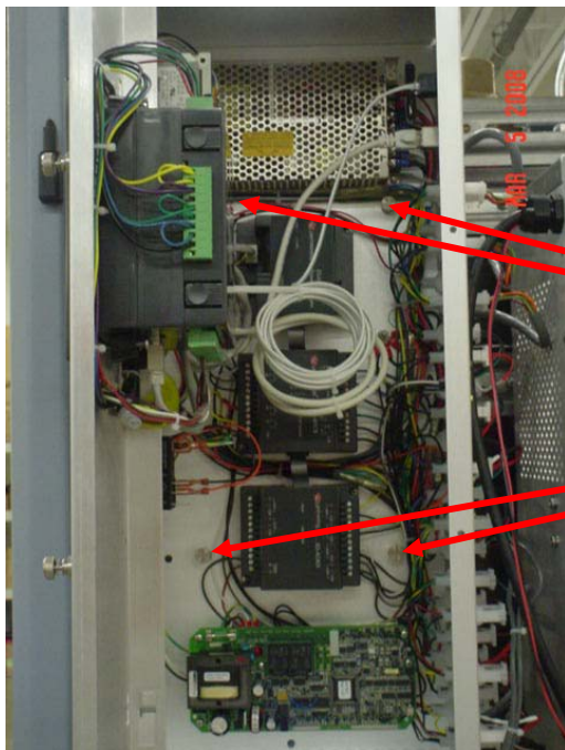
Photo 1 Signal Box interior- thumbscrew location
