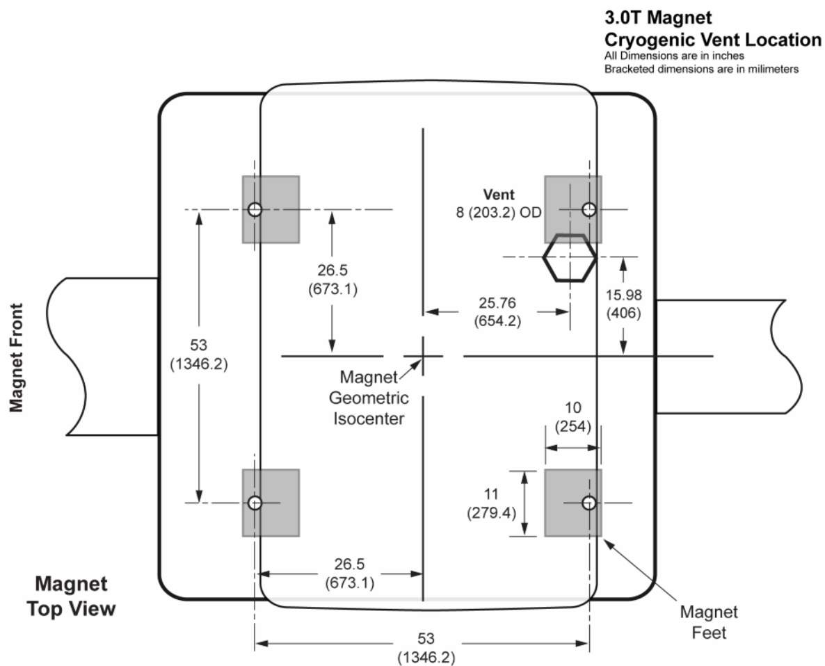
Illustration 3-12: Magnet Cryogenic Vent Location
