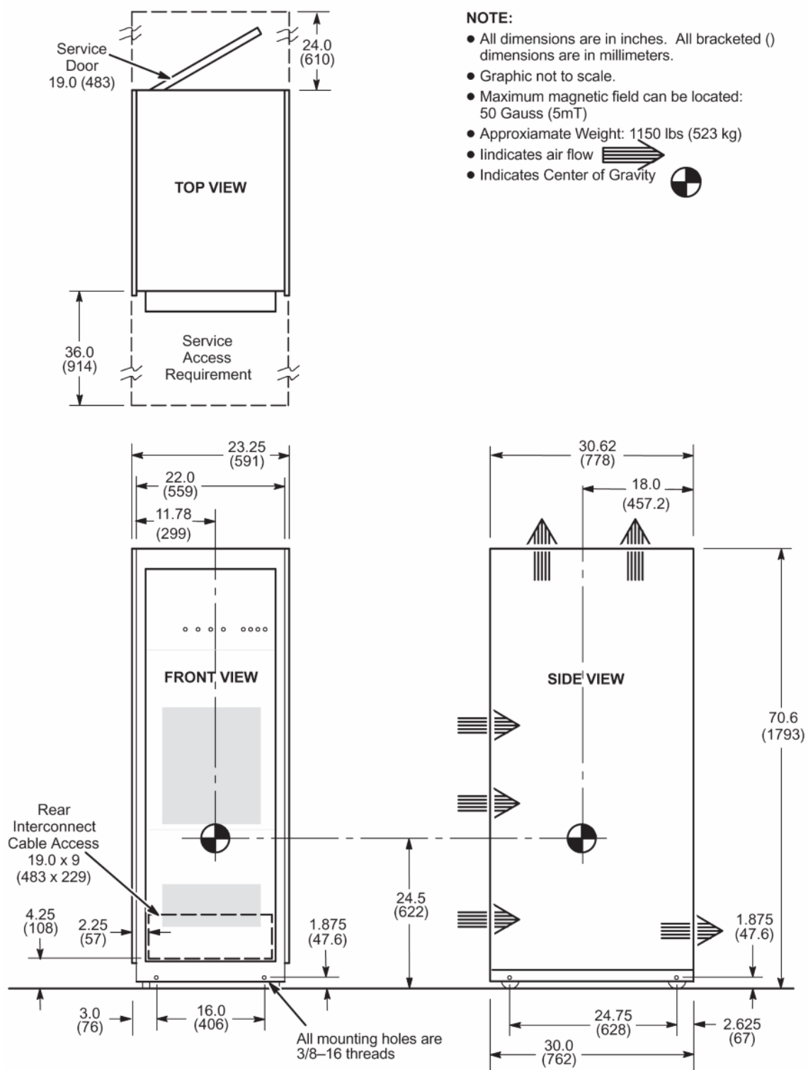
Illustration 4-10: MNS Amplifier Cabinet (MNS) for 8 kW MNS Option
