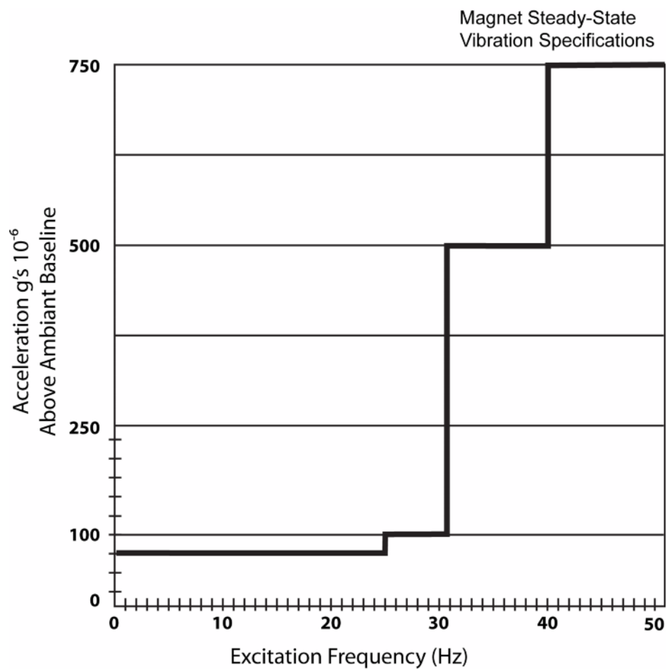
Illustration 3-2: Magnet Steady State Vibration Specifications
