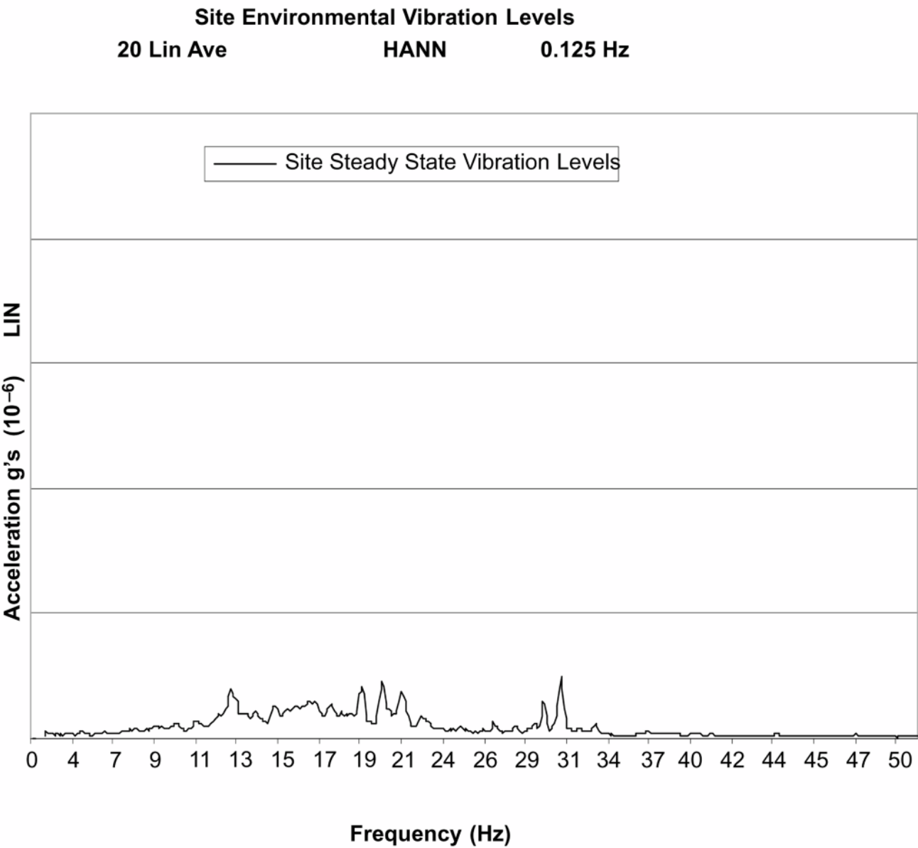
Illustration 7-1: Example of Site Environmental Vibration Levels
