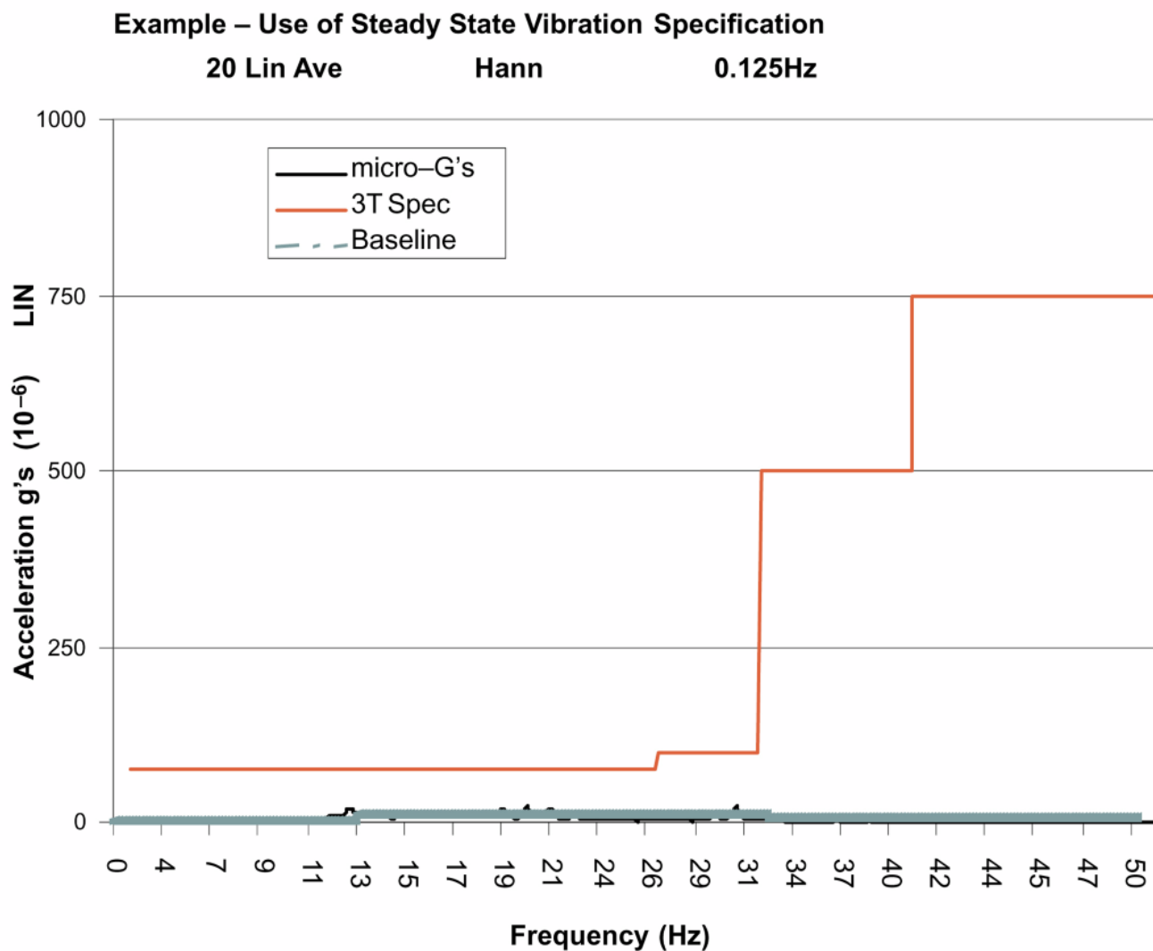
Illustration 7-2: Example Site Environmental Vibration
