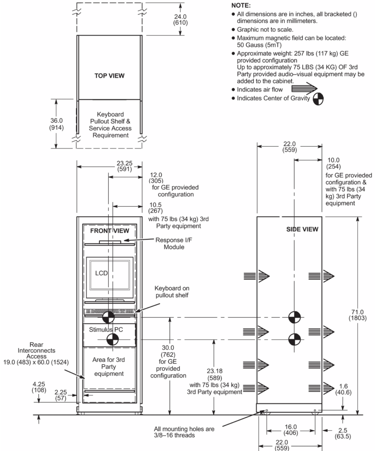
Illustration 4-11: Brainwave Lite Cabinet (BW)
