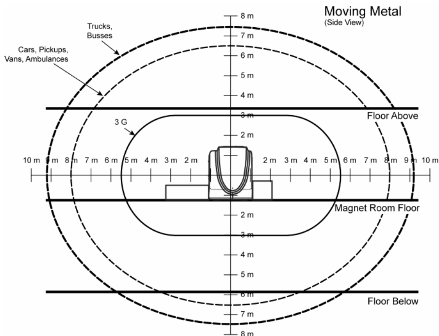
Illustration 2-8: Magnet Moving Metal Sensitivity Line Plot (Side View)
