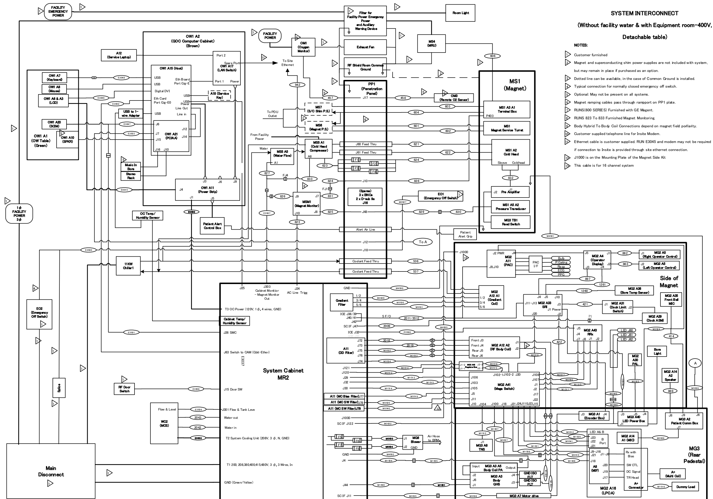
1-3 Cable map (Type C Detachable Table)
