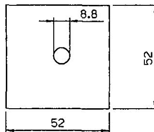
TYPE B1
