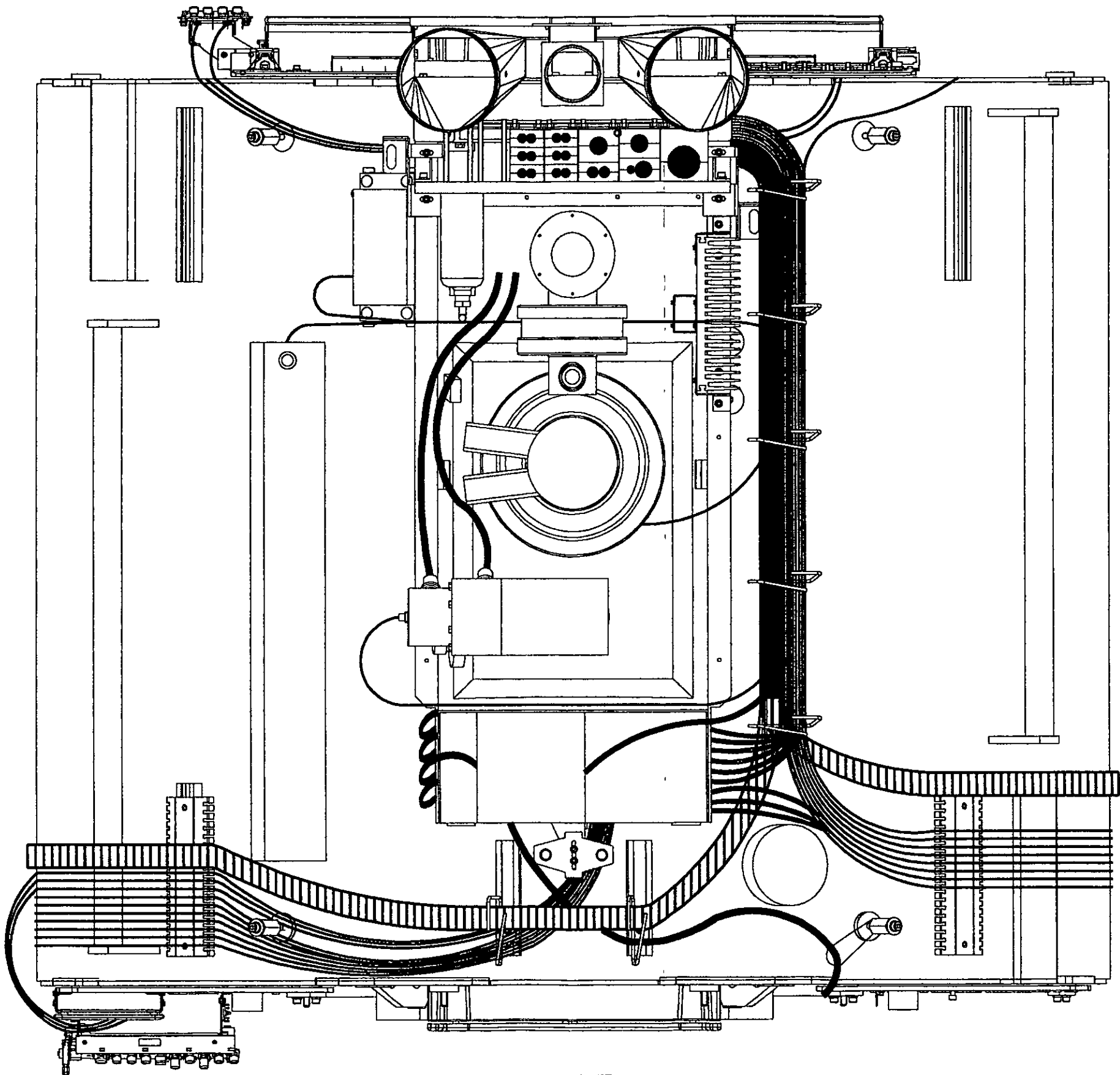
TOP VIEW
