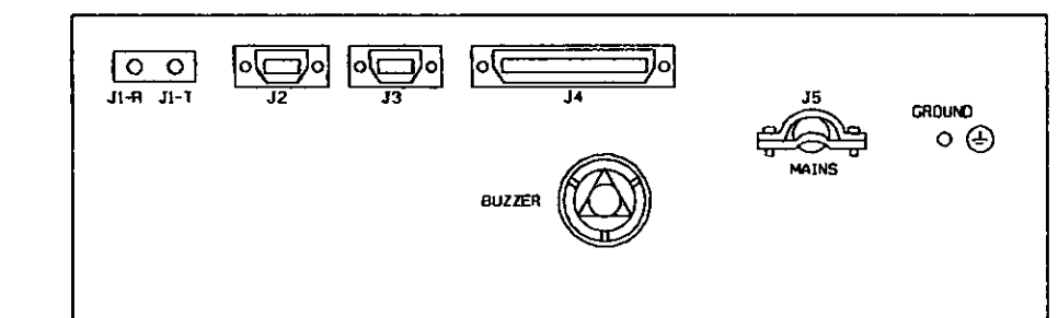
BOTTEM VIEW
