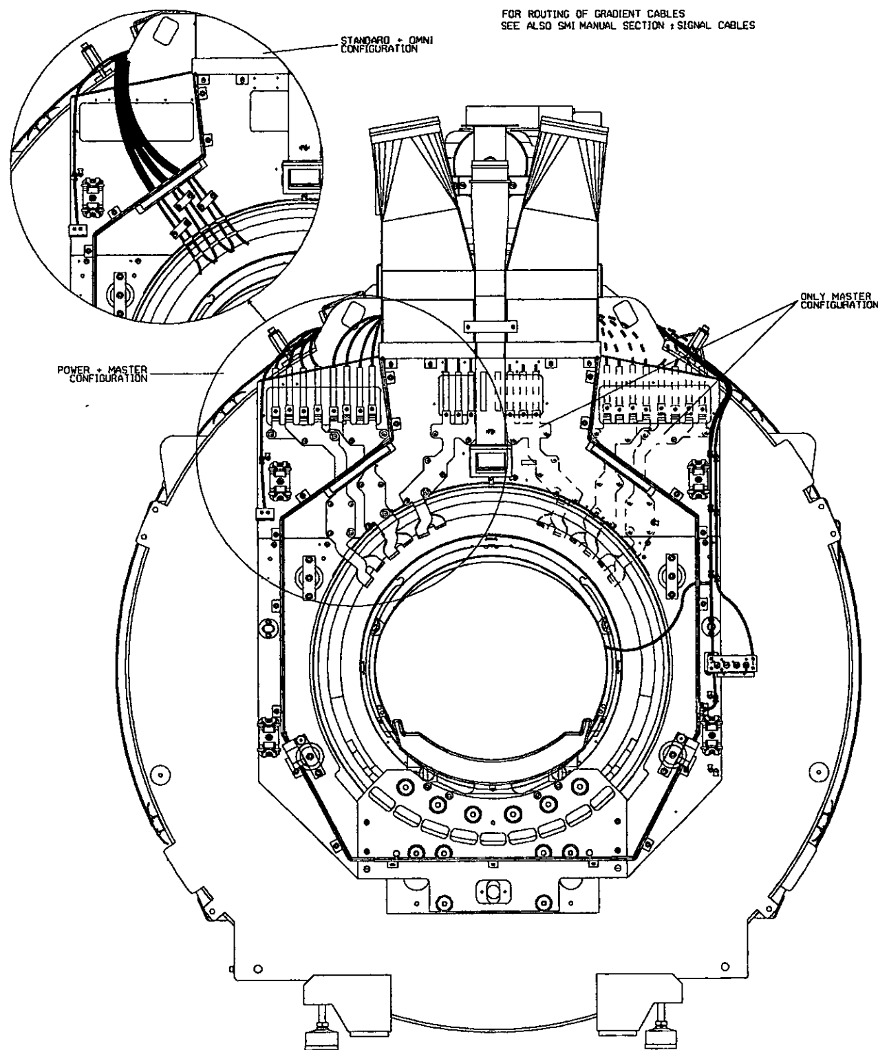
REAR VIEW
