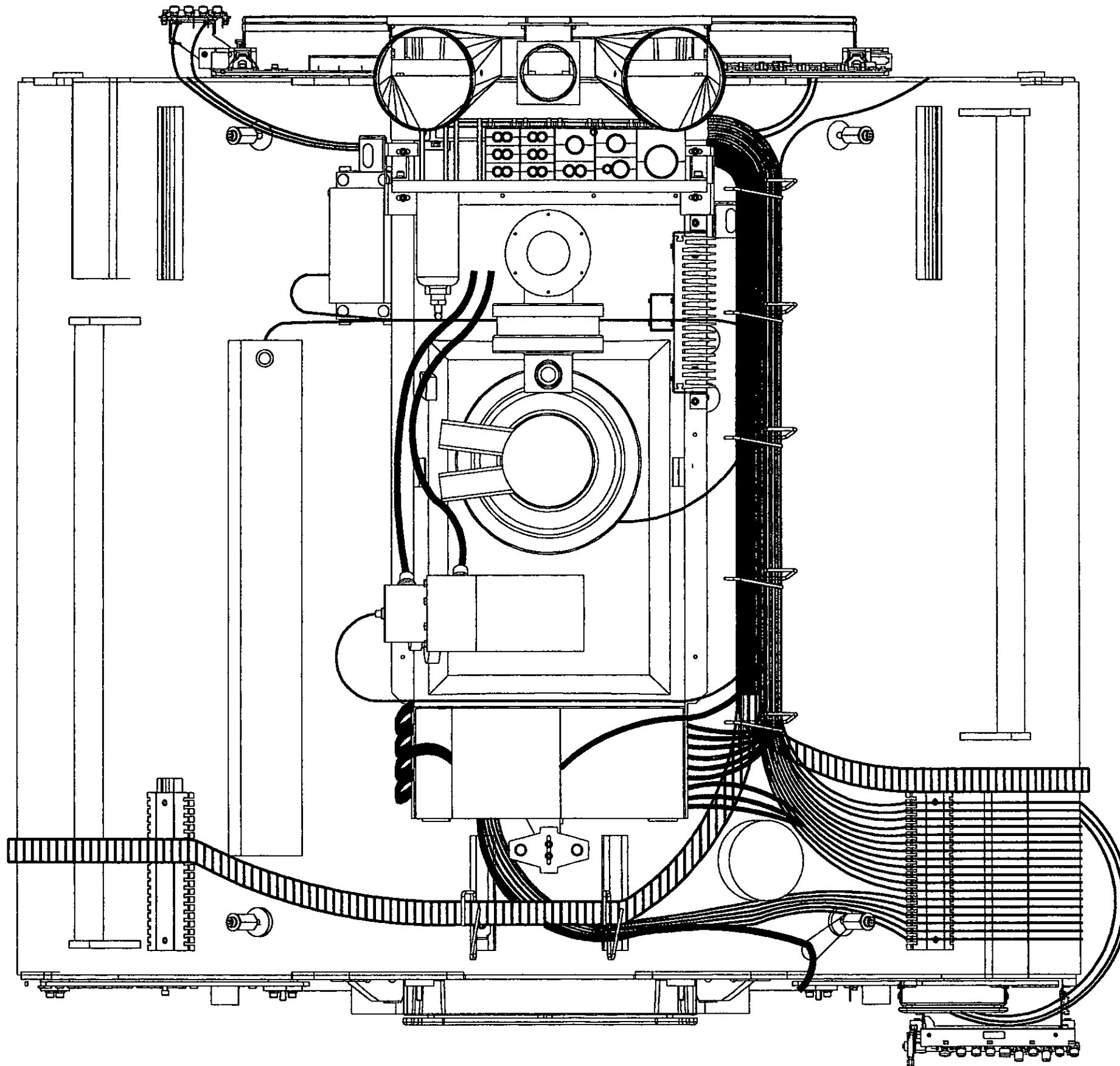
TOP VIEW
