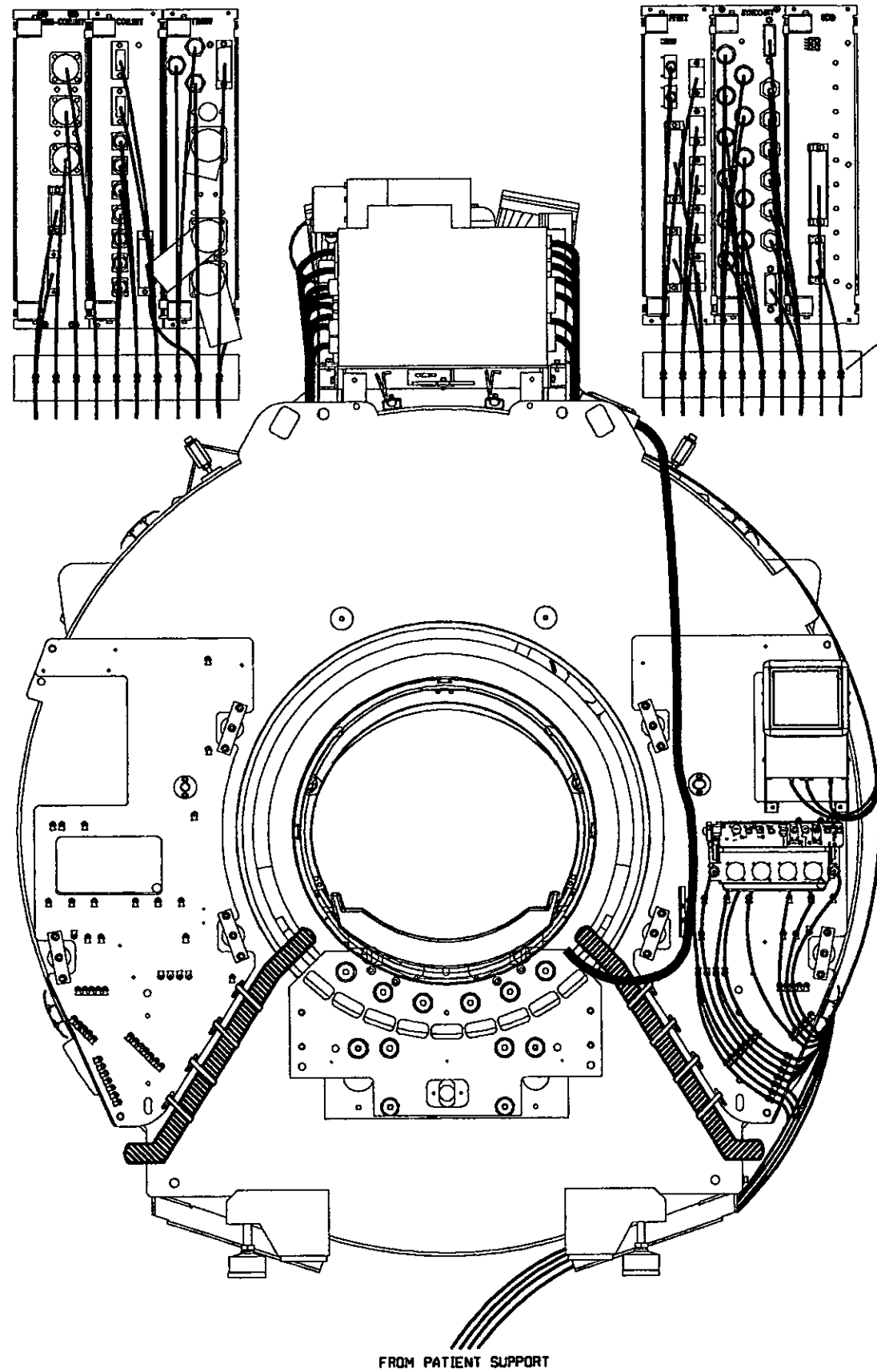
FRONT VIEW
