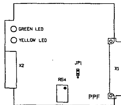
PERIPHERAL PULSE INTERFACE
