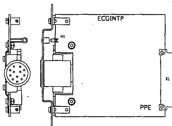
ECG INTERFACE (OPTIONAL) (4522 117 4766.)
