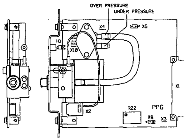
RESPIRATORY INTERFACE (4522 117 4778.)
