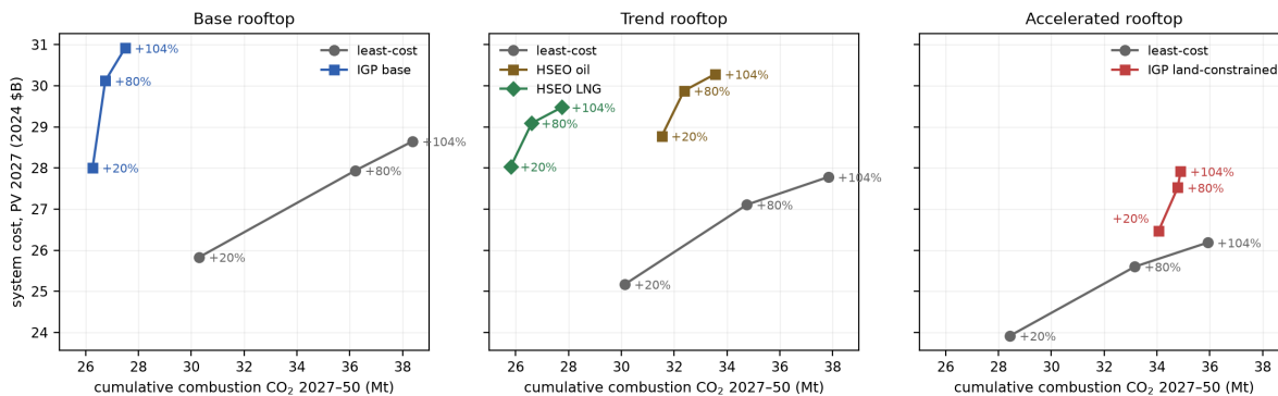
Figure 4.5 — Published plans against the least-cost path as the solar premium rises. Each panel is one rooftop trajectory. Each point is a solved cell: present-value system cost (2024$ billions) against cumulative combustion CO 2 over 2027–2050, at utility-solar premiums of 20, 80, and 104 percent over the mainland benchmark. Gray is the least-cost build on the same settings; colors are the plan-constrained cells. The plans sit near-vertical because their generation mixes are pinned, so higher solar costs raise their price without changing their emissions; the least-cost path slopes because the optimizer substitutes toward fossil generation as solar gets dearer.
