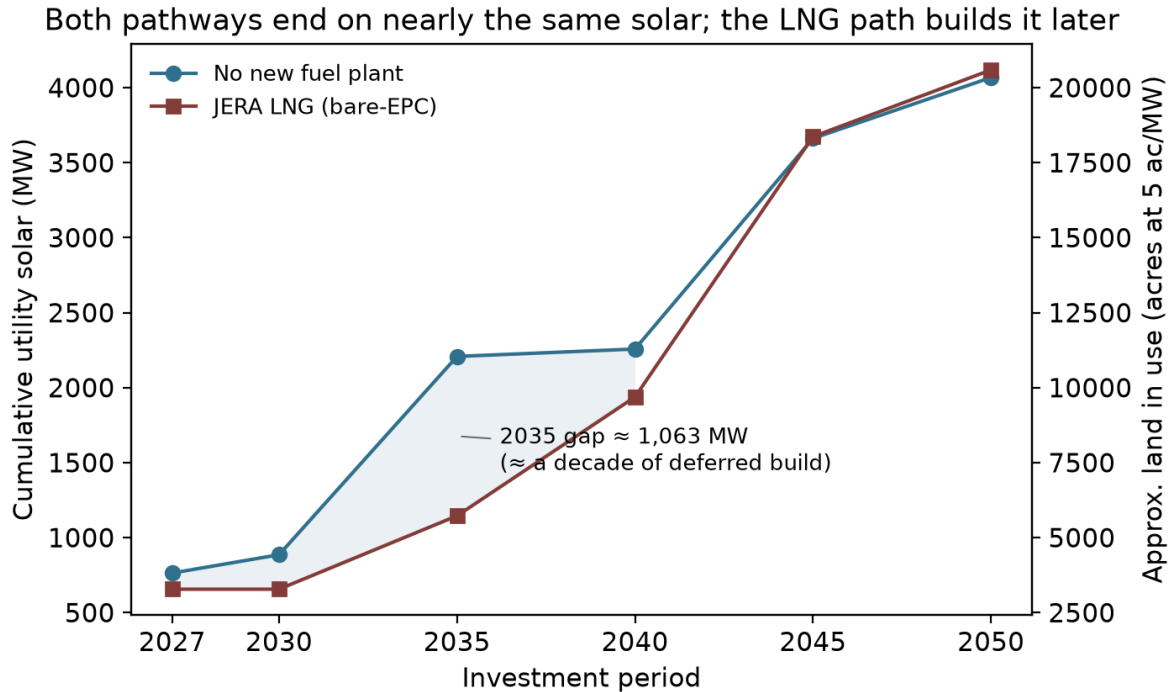
Figure 2.1 — Cumulative utility-scale solar on the no-new-plant and JERA LNG pathways. Cumulative installed utility-scale solar (MW, left axis; approximate land in use at five acres per megawatt, right axis) by investment period, at reference oil prices. The pathways end near the same total; the shaded area marks the build the LNG path defers, roughly a decade’s worth centered on 2035.
