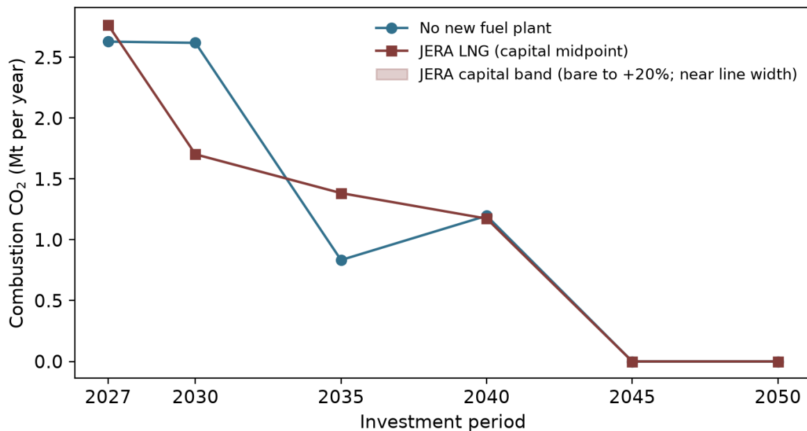
Annual combustion emissions: LNG cleaner around 2030, dirtier mid-2030s; cumulative totals in Section 4.7
