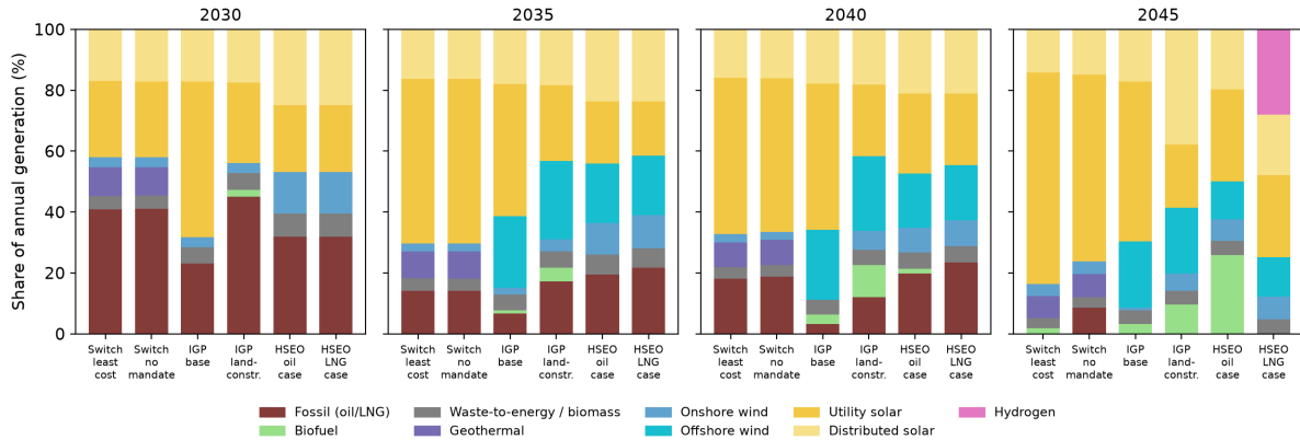
Figure 4.4 — Generation mix at anchor years: this report's least-cost and no-mandate paths (labeled “Switch” after the model; base rooftop trajectory, reference oil) against Hawaiian Electric’s Integrated Grid Plan (Figure 2-3 of the May 2023 final report). The IGP plans are named here by scenario — base and land-constrained — because the utility reversed which one it called “preferred”: the May 2023 report gave that label to the base scenario, and the November 2023 Supplemental Response moved it to the land-constrained scenario, which is now the plan of record. The HSEO study’s oil and LNG cases are drawn from the study’s own results worksheets (vended in sources/plan_mix/ ). Shares include customer-sited solar; the oil shares quoted in Section 2.7 are of grid supply alone and run a few points higher. In our solves, thermal generation with zero dispatch emissions is counted as biodiesel.
