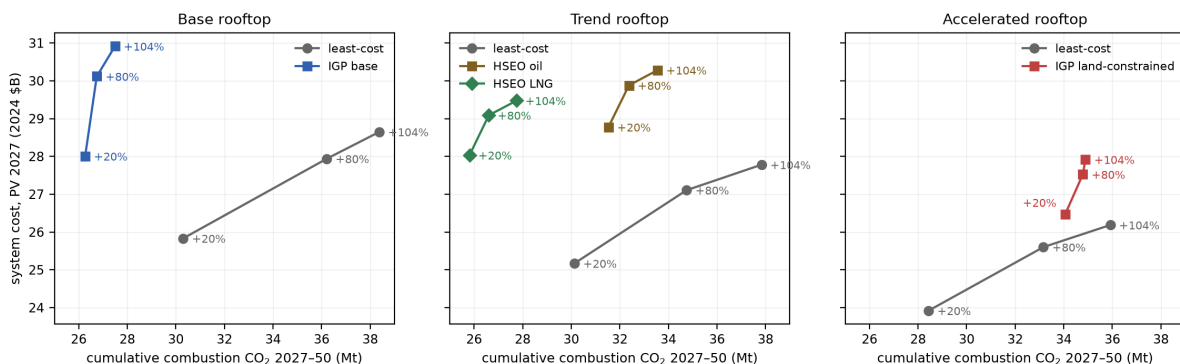
Figure 4.5 — Published plans against the least-cost path as the solar premium rises. Each panel is one rooftop trajectory. Each point is a solved cell: present-value system cost (2024$ billions) against cumulative combustion CO 2 over 2027–2050, at utility-solar premiums of 20, 80, and 104 percent over the mainland benchmark. Gray is the least-cost build on the same settings; colors are the plan-constrained cells. The plans sit near-vertical because their generation mixes are pinned, so higher solar costs raise their price without changing their emissions; the least-cost path slopes because the optimizer substitutes toward fossil generation as solar gets dearer.
