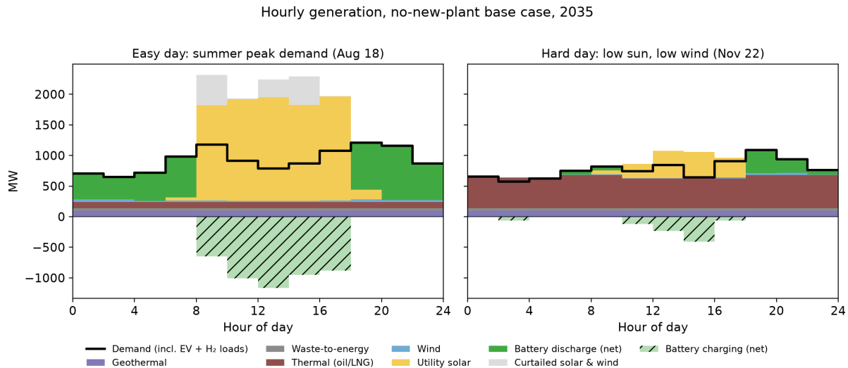
Figure 5.1 — Hourly dispatch on the two 2035 sample days, no-new-plant base case. Stacked generation (MW) by two-hour model timepoint on the summer peak-demand day (August 18) and the low-sun, low-wind day (November 22), rendered as in the results explorer. The black step line is demand; the hatched bars below zero are net battery charging; the gray band is curtailed solar and wind, potential output above what was dispatched. Battery flows are shown net: in surplus hours the optimizer may charge and discharge simultaneously, a costless way to shed surplus, which the net view removes; the round-trip losses of that disposal are counted as curtailment. Generation sources stack in the legend's order.
