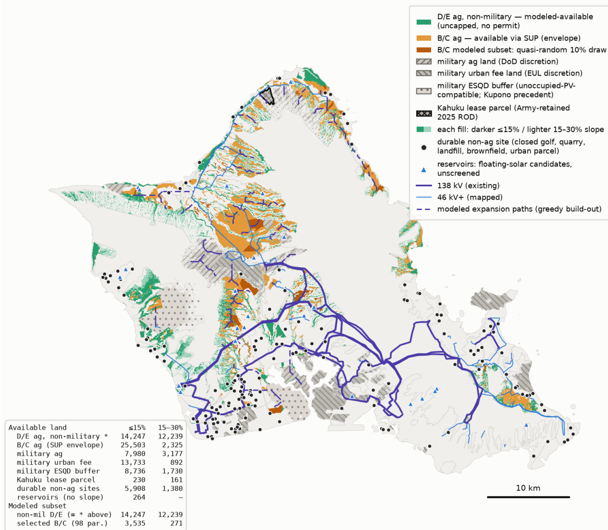
Figure 2.3 — Plausibly available solar land, the modeled subset, and the transmission network. Land plausibly available for utility-scale solar, colored by tenure and legal pathway: uncapped Class D/E agricultural land (modeled as available), the Class B/C envelope reachable by special use permit together with the quasi-random 10 percent draw the model uses, military lands by discretion category, durable non-agricultural sites (closed golf courses, quarries, landfills, brownfields), and reservoir surfaces (floating-solar candidates). Within each category, darker fill marks slopes of 15 percent or less and lighter fill 15–30 percent. Purple lines are the existing 138 kV and mapped 46 kV-plus network; dashed lines are modeled expansion paths. The inset table gives acreage by category and slope band; the modeled subset totals about 30,300 acres.
