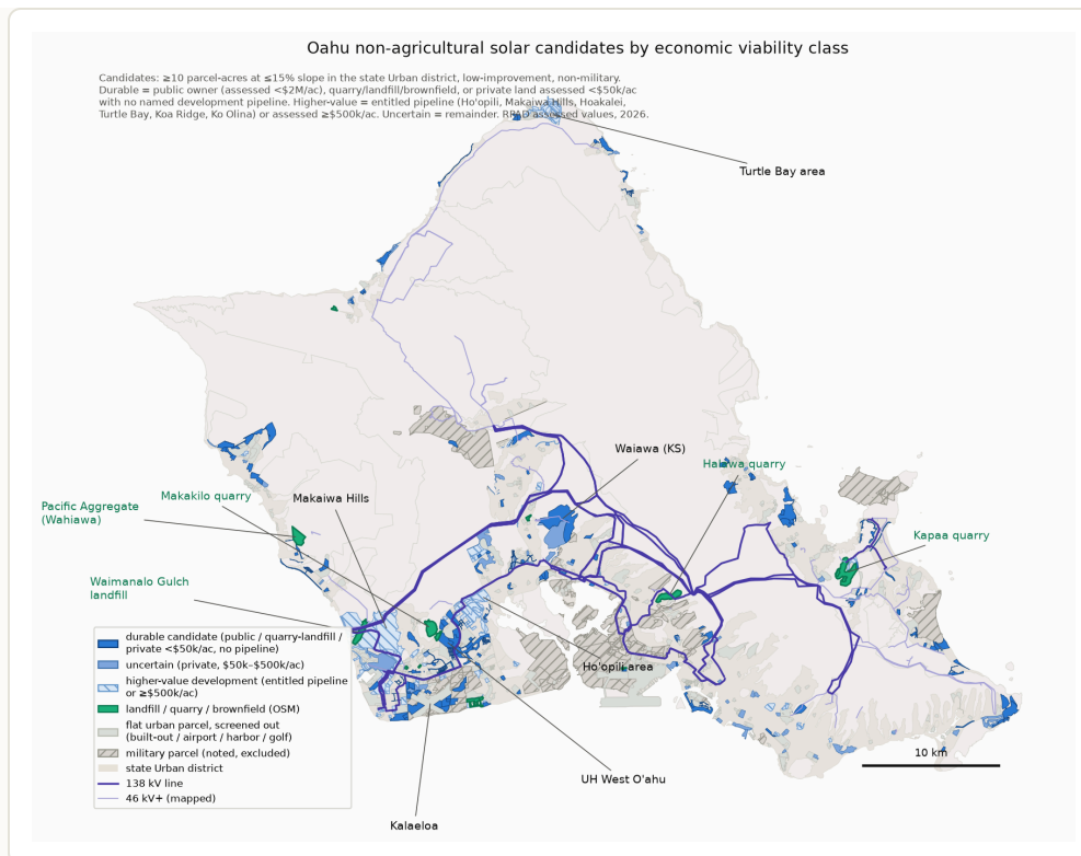
Figure 9. Non-agricultural solar candidates: low-improvement urban-district parcels ( \geq 10 ac at \leq 15\% slope, non-military), screened-out flat urban parcels, military land (noted, excluded), and landfill/quarry/ brownfield sites, with mapped transmission. Improvement-value proxy and OSM site inventory carry the caveats in the notes file.
