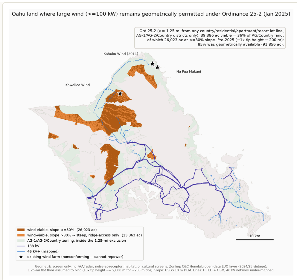
Figure 10. Wind-viable land under Ordinance 25-2: AG/Country zoning beyond 1.25 miles of any country/residential/apartment/resort-district lot, toned by slope, with the three existing (non-repowerable) wind farms marked. Geometric screen only — no FAA/radar, noise-at-receptor, habitat, or cultural screens.
