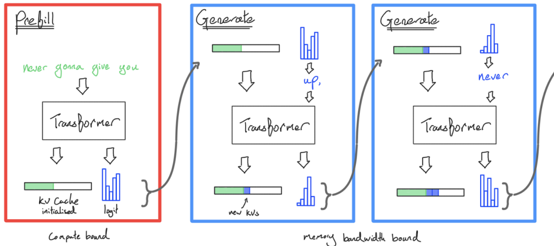
Figure: diagram of efficient Transformer sampling with a KV cache.
