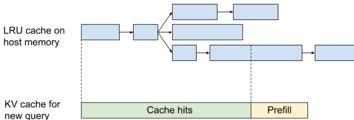
Figure: KV prefix cache implemented as an LRU trie. We can avoid duplicating KV memory by sharing prefixes. Source:
