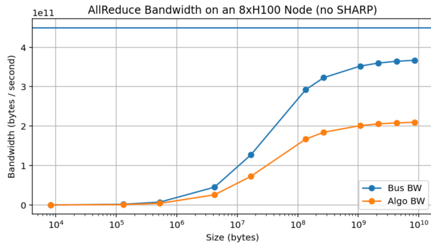
Figure: AllReduce throughput for an 8xH100 node with SHARP disabled. The blue curve is the empirical link bandwidth, calculated as (2 * \text{bytes} * (N - 1) / (N * \text{runtime})) from the empirical measurements. Note that we do not get particularly close to the claimed bandwidth of 450GB/s, even with massive 10GB arrays.
