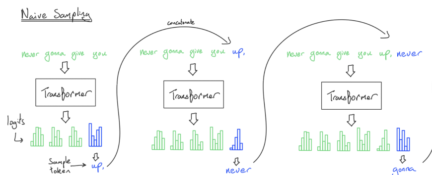
Figure: naive sampling from a Transformer. The blue logits give us a distribution over the next token that we can sample from. Note that each step re-processes
