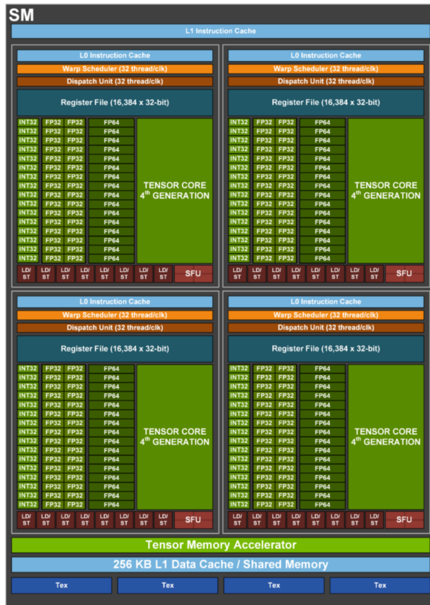
Figure: a diagram of an H100 SM (source) showing the 4 subpartitions, each containing a Tensor Core, Warp
