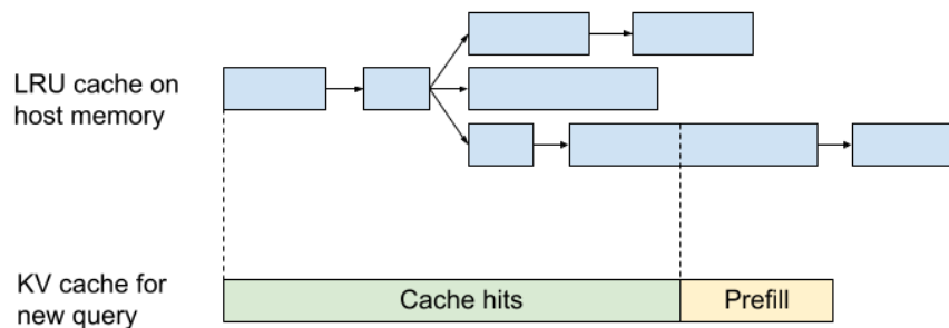
Figure: KV prefix cache implemented as an LRU trie. We can avoid duplicating KV memory by sharing prefixes. Source: Character.ai blog.
