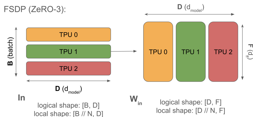
Figure: FSDP shards the contracting dimension of W_{in} and the output dimension of W_{out} along the data
