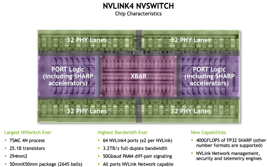
Figure: a lower level view of a single NVLink4 Switch.
