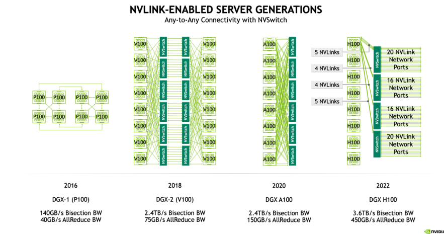
Figure: node aka NVLink domain diagrams from Pascal (P100) onward. Since Volta (V100), we have had all-to-all connectivity within a node using a set of switches. The H100 node has 4 NVSwitches connected to all 8 GPUs with 25GB/s links.
