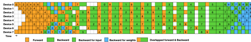
Figure: the DeepSeek v3 pipeline schedule (from their recent paper). Orange is the forward matmul, green is the dL/dx matmul, and blue is the dL/dW matmul. By prioritizing the backwards dL/dx multiplications, we can avoid "stranding" FLOPs.
