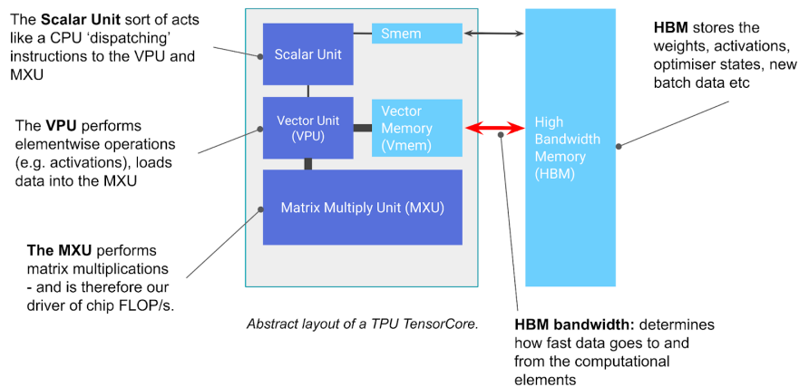
Figure: the basic components of a TPU chip. The TensorCore is the gray left-hand box, containing the matrix-multiply unit (MXU), vector unit (VPU), and vector memory (VMEM).
