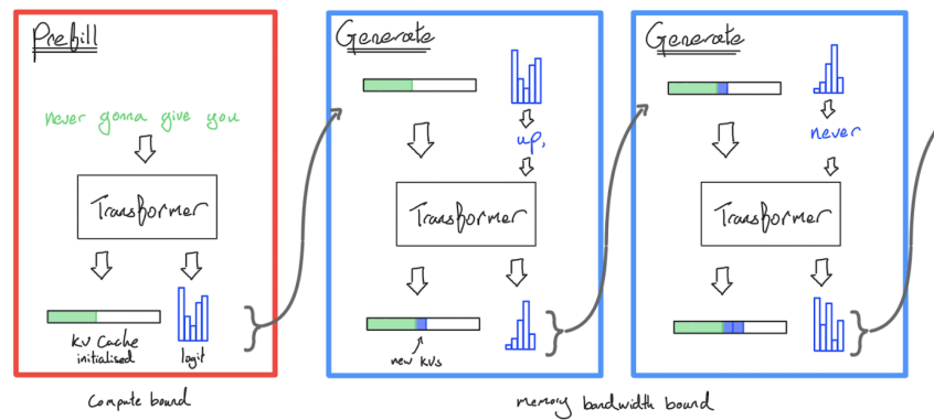
Figure: diagram of efficient Transformer sampling with a KV cache. Prefill processes our prompt and saves all the per-token key-value activations in a cache.
