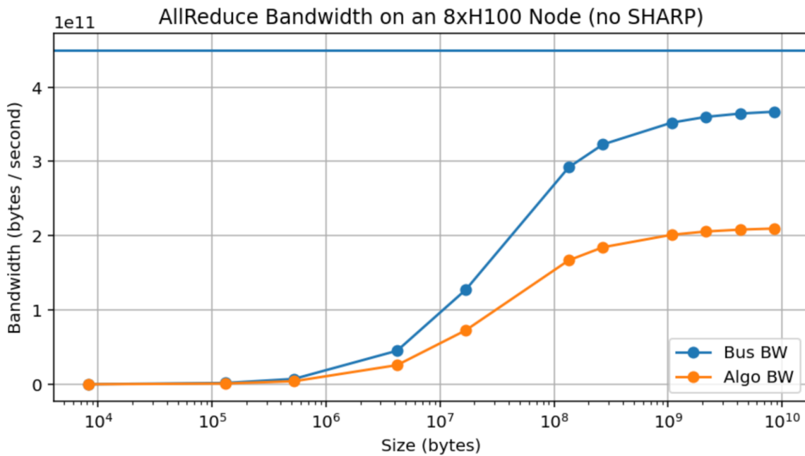
Figure: AllReduce throughput for an 8xH100 node with SHARP disabled. The blue curve is the empirical link bandwidth, calculated as 2 \cdot \text{bytes} \cdot (N - 1) / (N \cdot \text{runtime}) from the empirical measurements. Note that we do not get particularly close to the claimed bandwidth of 450GB/s, even with massive 10GB arrays.
