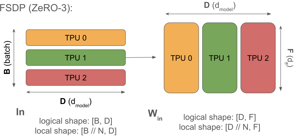
Figure: FSDP shards the contracting dimension of W_{\text{in}} and the output dimension of W_{\text{out}} along the data dimension. This reduces memory but (from Section 3) requires us to gather the weights for W before we perform the matmul. Note that the activations (left) are not sharded along the contracting dimension, which is what forces us to gather. Note that our weight optimizer state is likewise sharded along the contracting dimension.
