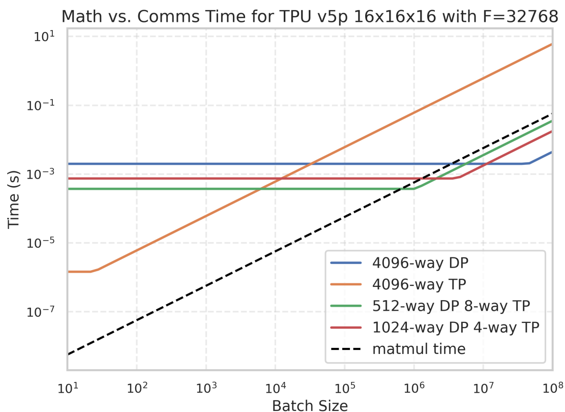
Figure: time taken for communication with different parallelism schemes. The black dashed line is the time taken by the matrix multiplication FLOPs, so any curve above this line is comms-bound. We note that all strategies become comms-bound below batch size 6e5 , which is in line with our expected 4096 * 2550^2 / (2 * 8192 * 4) = 4e5 .
