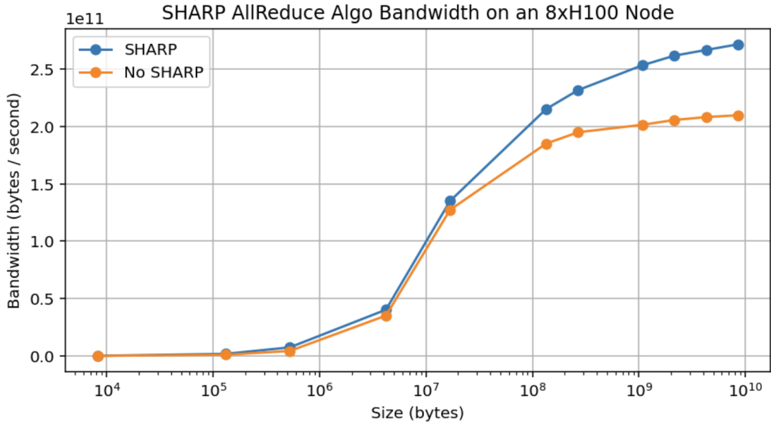
Figure: empirical measurements of AllReduce algo bandwidth with and without NVIDIA SHARP enabled within a node. The gains amount to about 30% throughput improvement at peak, even though algorithmically it ought to be able to achieve closer to a 75% gain.
