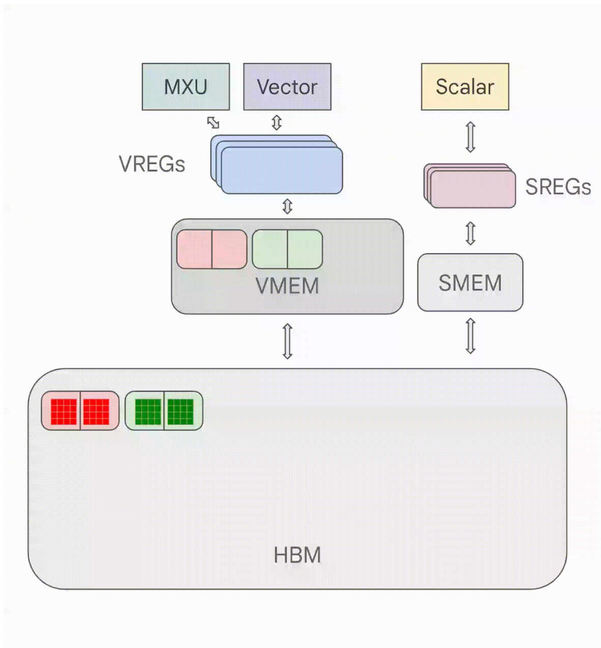
Figure: a diagram from Section 2 showing how a TPU performs an elementwise product. Depending on the size of our arrays and the bandwidth of various links, we can find ourselves compute-bound (using the full hardware compute capacity) or comms-bound (bottlenecked by memory loading).
