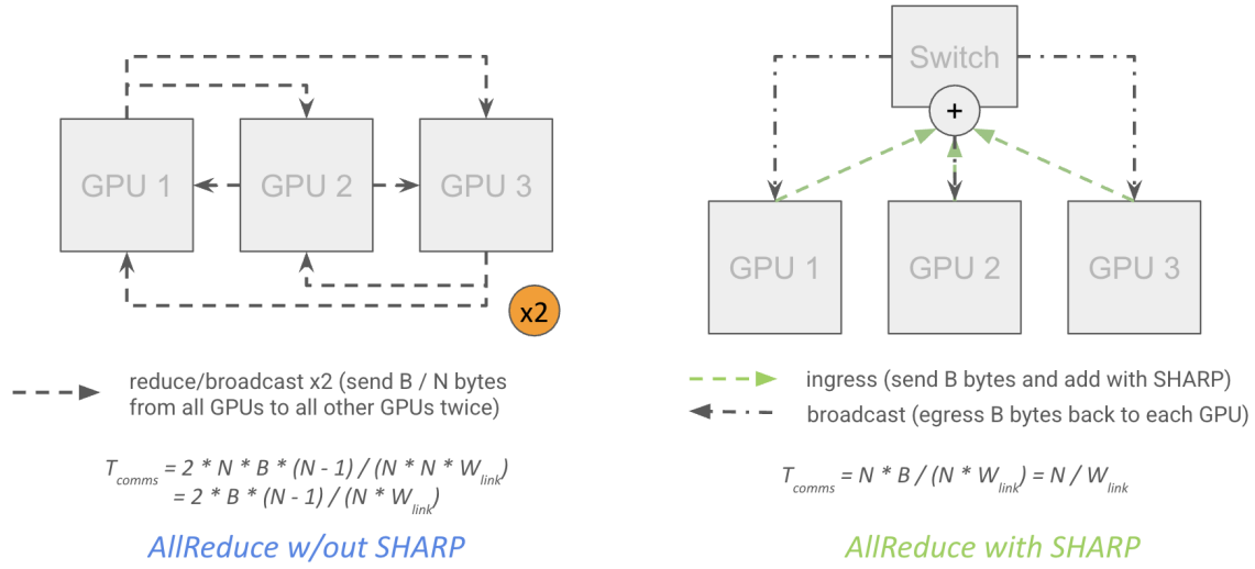
Figure: an AllReduce without SHARP has 2x the theoretical cost because it has to pass through each GPU twice. In practice, speedups are only about 30% (from NCCL 2.27.5).
