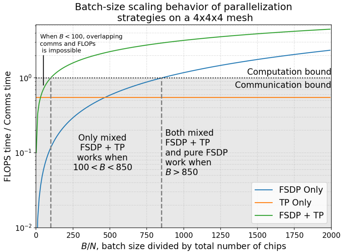
Figure: ratio of FLOPs to comms time for optimal mixed FSDP/TP on a TPUv5p 4x4x4 slice with F=30k . As expected, tensor parallelism has a fixed ratio with batch size; ideal mixed FSDP + TP scales with B , and FSDP scales with B . However, in intermediate batch size regimes, only FSDP + TP achieves a ratio greater than unity.
