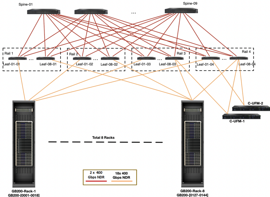
Figure: a diagram showing a GB200 DGX SuperPod of 576 GPUs.
