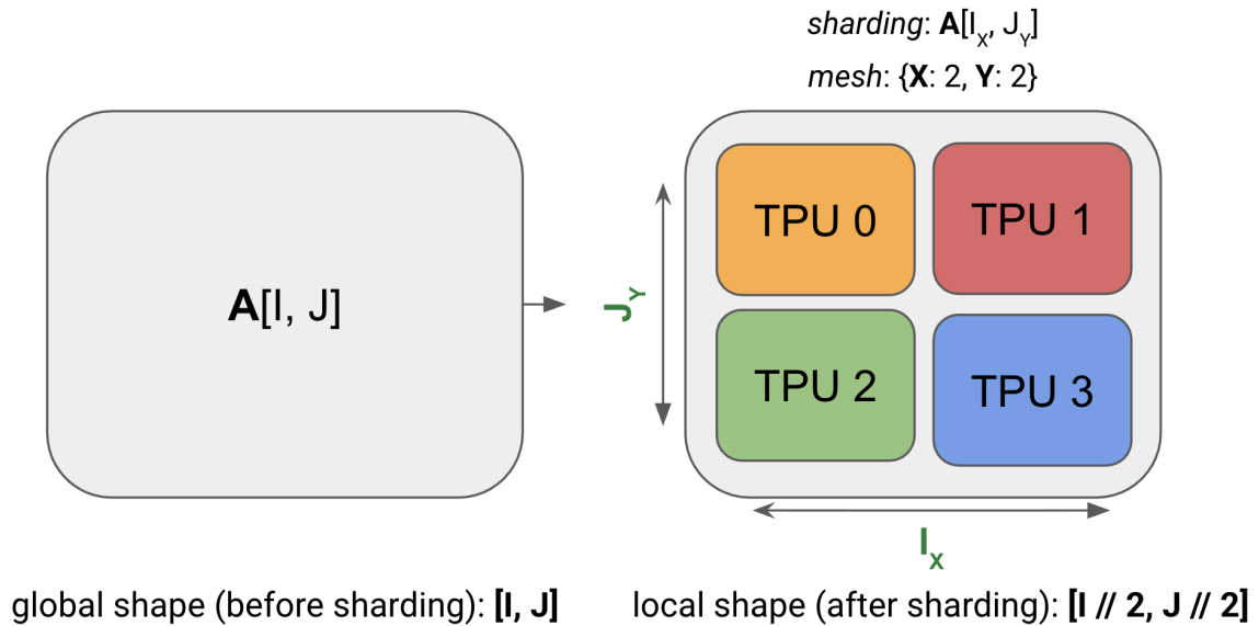
Figure: an example array of shape A[I, J] gets sharded across 4 devices. Both dimensions are evenly sharded across 2 devices with a sharding A[I_x, J_y] . Each TPU holds 1/4 of the total memory.
