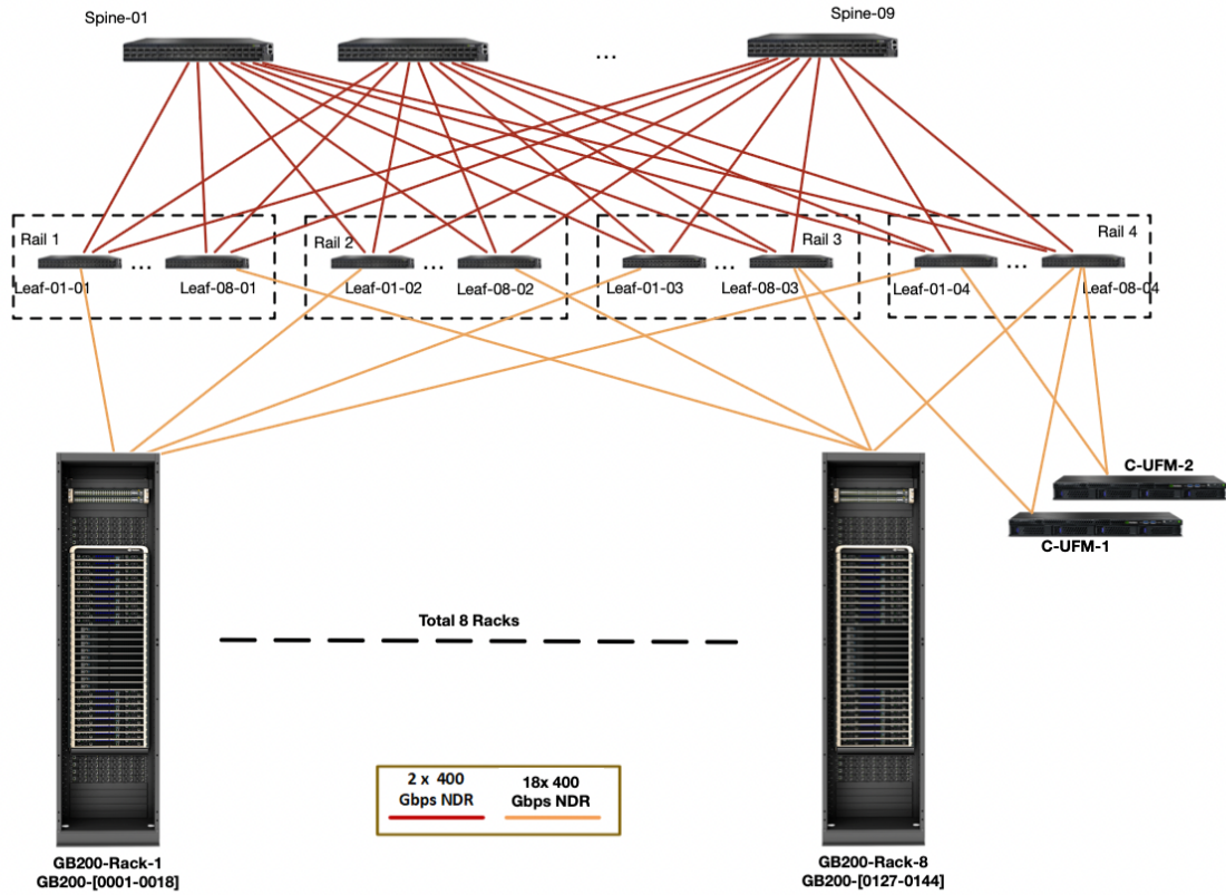
Figure: a diagram showing a GB200 DGX SuperPod of 576 GPUs. Each rack at the bottom layer contains 72 GB200 GPUs.
