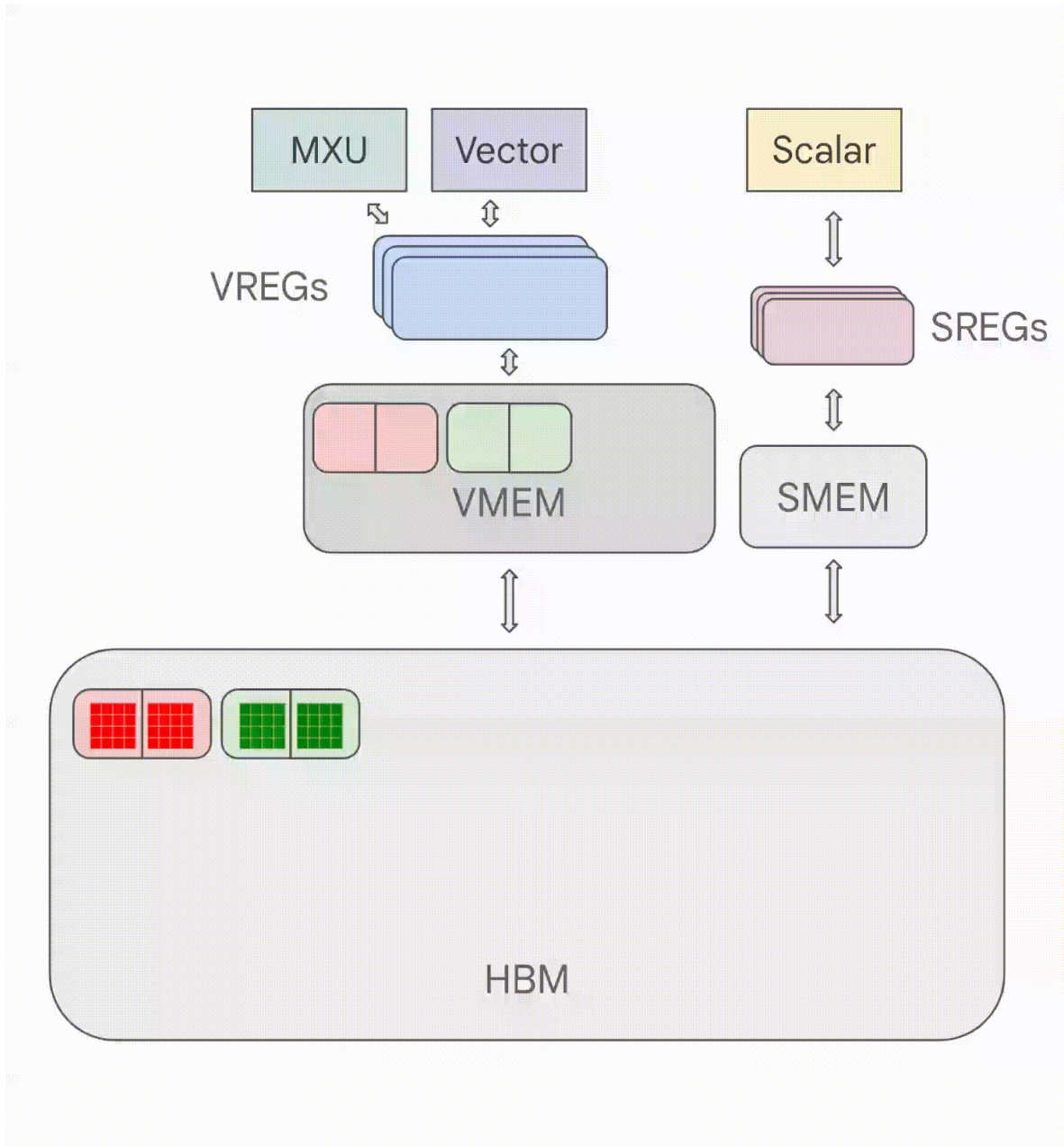
Figure: an animation showing a pointwise product performed on TPU, with bytes loaded from HBM. Note how bytes are streamed out of memory in chunks and partial results are pipelined back without waiting for the full array to be materialized.
