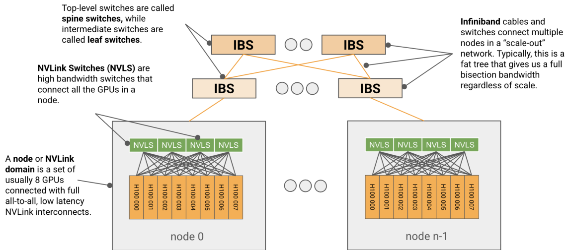
Figure: a diagram showing a typical H100 network. A set of 8 GPUs is connected into a node or NVLink domain with NVSwitches (also called NVLink switches), and these nodes are connected to each other with a switched InfiniBand fabric. H100s have about 450GB/s of egress bandwidth each in the NVLink domain, and each node has 400GB/s of egress bandwidth into the IB network.
