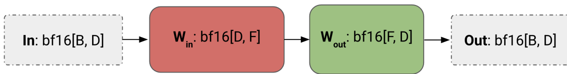
Figure: a simplified Transformer layer. We treat each FFW block as a stack of two matrices W_{\text{in}}: \text{bf16}[D, F] (up-projection) and W_{\text{out}}: \text{bf16}[F, D] (down-projection) with an input \text{In}: \text{bf16}[B, D] .
