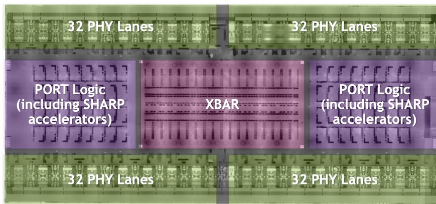
NVLink4 NVSWITCH Chip Characteristics
