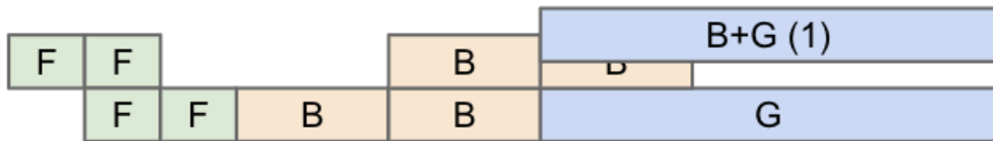
Figure: an example 2 stage, 2 microbatch pipeline. F denotes a stage forward pass and B is a stage backward pass (2x the cost). G denotes the data-parallel AllReduces, which can be significantly longer than the time of a single microbatch.
