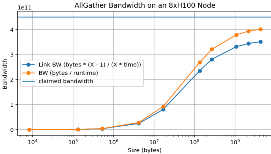
Figure: AllGather bandwidth on an 8xH100 cluster (intra-node).
