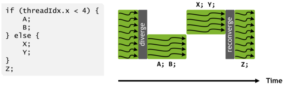
Figure: an example of warp divergence within a set of threads ( source ). White spaces indicate stalls of at least some fraction of the physical CUDA cores
