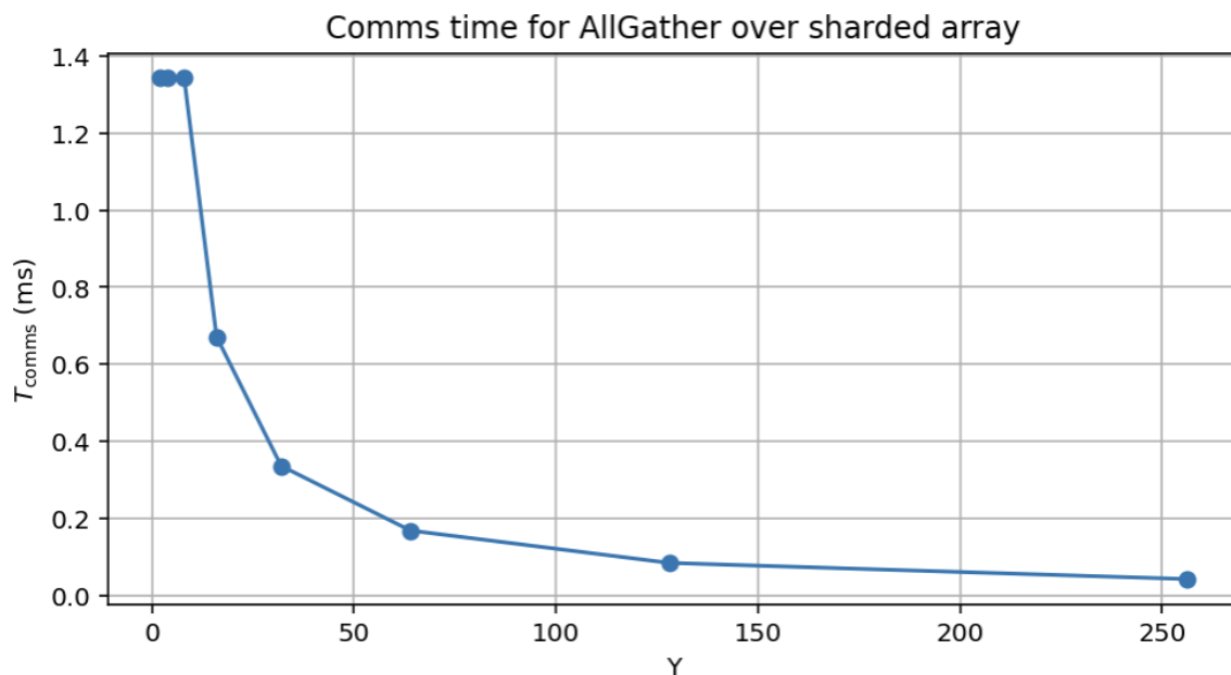
Figure: theoretical cost of a sharded AllGather as the inner axis spans more nodes.
