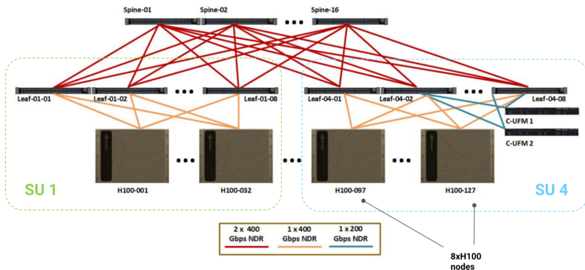
Figure: diagram of the reference 1024 H100 DGX SuperPod with 128 nodes (sometimes 127), each with 8 H100 GPUs, connected to an InfiniBand scale-out network. Sets of 32 nodes (256 GPUs) are called 'Scalable Units' or SUs. The leaf and spine IB switches provide enough bandwidth for full bisection bandwidth between nodes.
