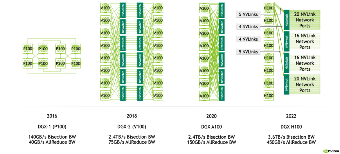
Figure: node aka NVLink domain diagrams from Pascal (P100) onward. Since Volta (V100), we have had all-to-all connectivity within a node using a set of switches. The H100 node has 4 NVSwitches connected to all 8 GPUs with 25GB/s links.
