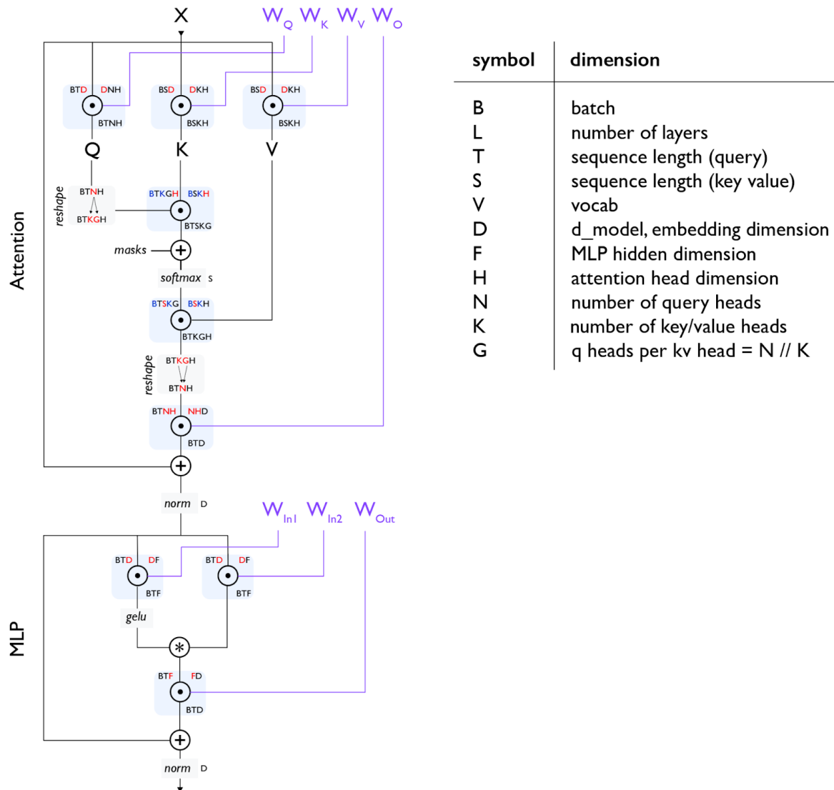
Figure: this diagram shows one layer of a standard Transformer and flows from top-to-bottom. We use a single-letter convention to describe the shapes and layouts of arrays in a Transformer, again showing contracting dimensions in red, and batched dimensions in blue. In a given operation, the input shape is given on top-left and the parameter shape is given on the top-right, with the resulting shape below, e.g. BTD is the input shape for the gating einsum and DF is the weight shape.
