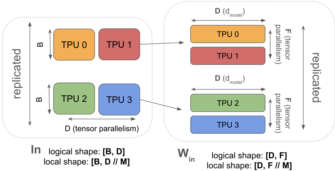
Figure: an example of basic tensor parallelism. Since we're only sharding our activations over Y (unlike in FSDP where we shard over X ), we replicate our activations over X . Using our standard syntax, this is A[B, D_Y] * B[D, F_Y] \rightarrow C[B, F_Y] . Because we're only sharding over one of the contracting dimensions, we typically AllGather the activations A before the matmul.
