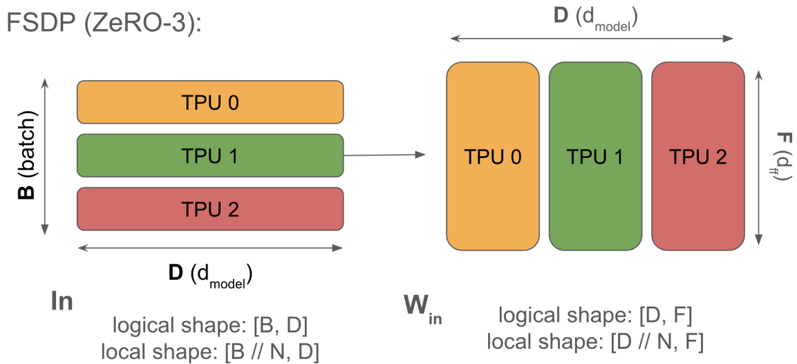
Figure: FSDP shards the contracting dimension of W_{\text{in}} and the output dimension of W_{\text{out}} along the data dimension. This reduces memory but (from Section 3) requires us to gather the weights for W before we perform the matmul. Note that the activations (left) are not sharded along the contracting dimension, which is what forces us to gather. Note that our weight optimizer state is likewise sharded along the contracting dimension.
