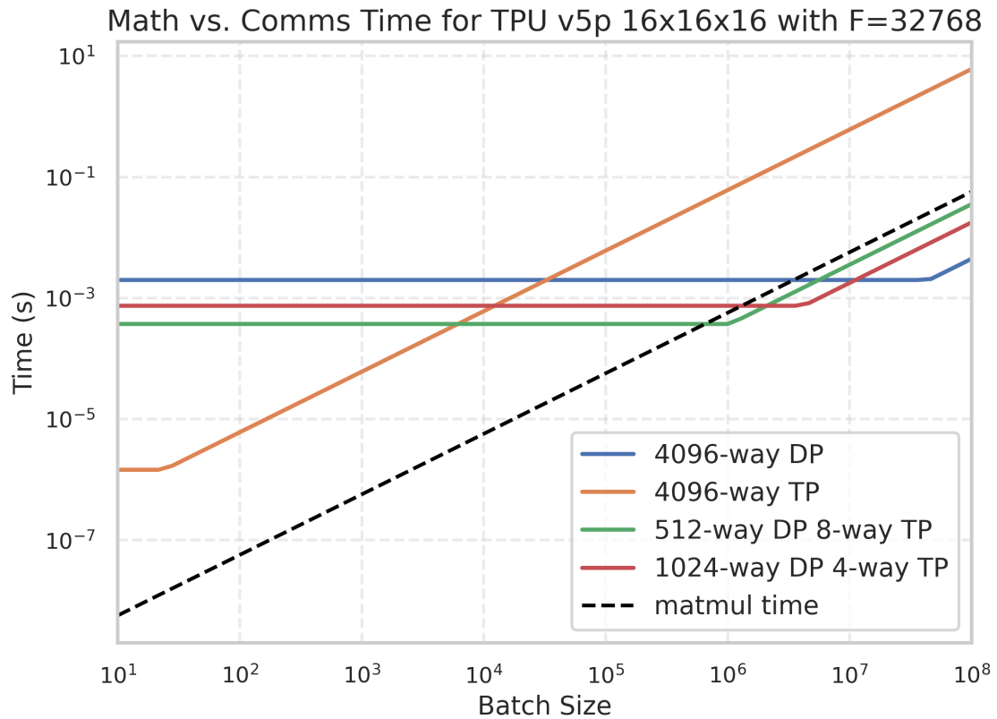
Figure: time taken for communication with different parallelism schemes. The black dashed line is the time taken by the matrix multiplication FLOPs, so any curve above this line is comms-bound. We note that all strategies become comms-bound below batch size 6e5 , which is in line with our expected 4096 * 2550^2 / (2 * 8192 * 4) = 4e5 .
