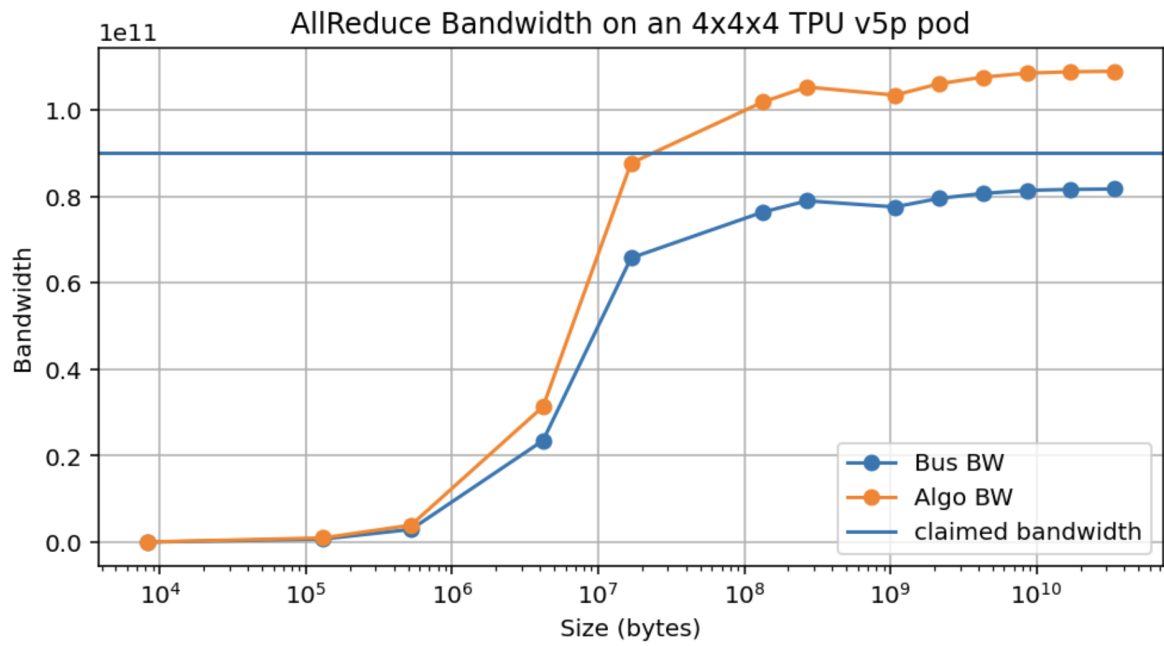
Figure: AllReduce bandwidth on a TPU v5p 4x4x4 cluster (along one axis).
