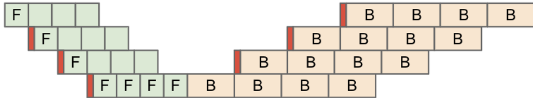
Figure: an example pipeline showing transfer cost in red. This shifts stages relative to each other and increases the pipeline bubble overhead.
