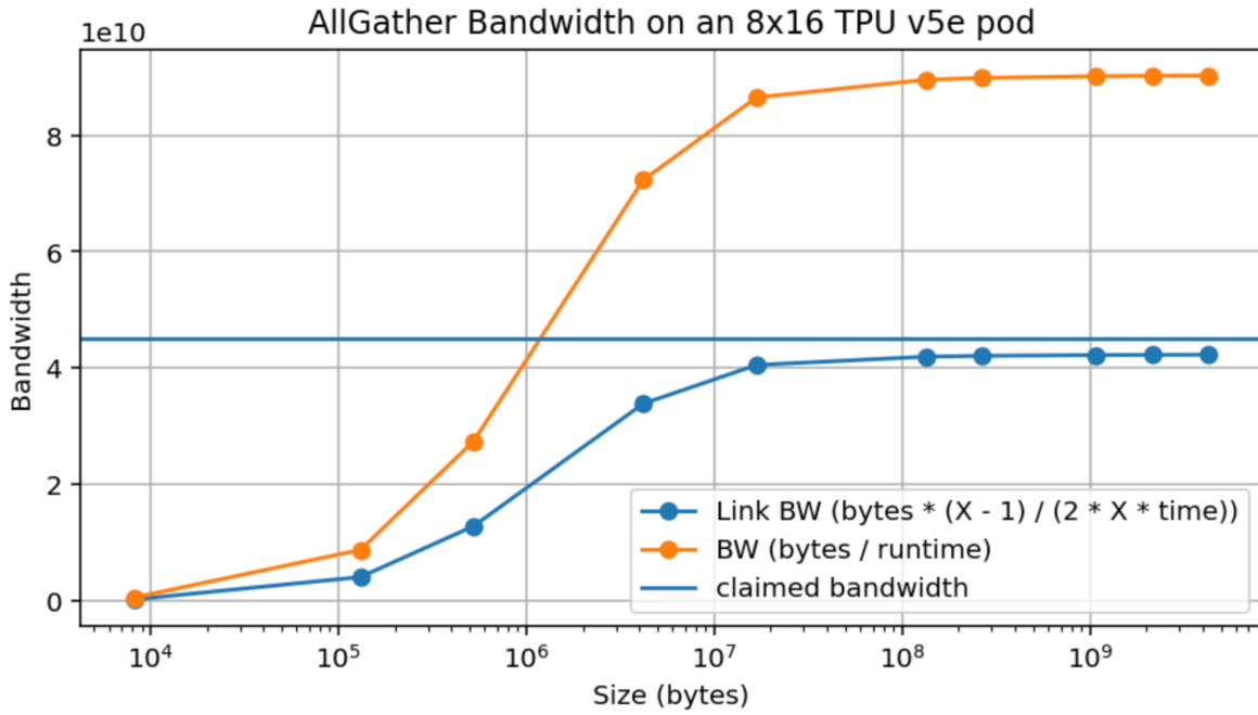
Figure: AllGather bandwidth on a TPU v5e 8x16 cluster (along one axis).
