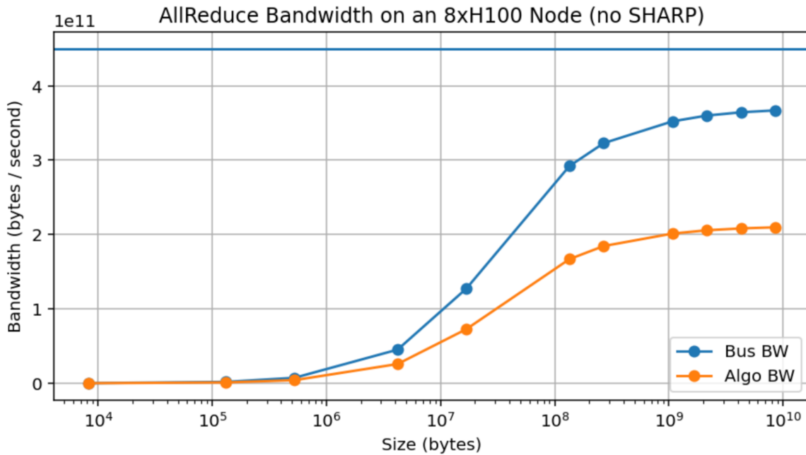
Figure: AllReduce throughput for an 8xH100 node with SHARP disabled. The blue curve is the empirical link bandwidth, calculated as 2 \cdot \text{bytes} \cdot (N-1) / (N \cdot \text{runtime}) from the empirical measurements. Note that we do not get particularly close to the claimed bandwidth of 450GB/s, even with massive 10GB arrays.
