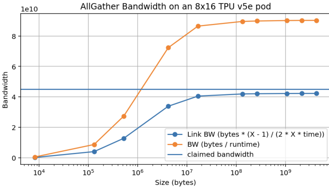
Figure: empirical bandwidth and estimated link bandwidth for TPU v5e during an AllGather. BW in orange is the actual bytes per second AllGathered, while the blue curve shows the empirical unidirectional link bandwidth calculated according to the known cost of the collective.
