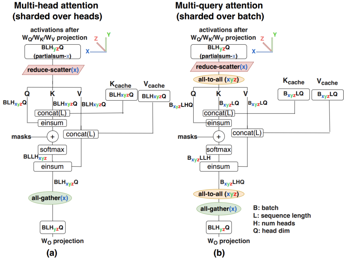
Figure: comparison of the attention mechanism with (a) Multi head attention with pure model sharding and (b) Multiquery attention with batch sharding of the KV cache. Notice how we need two extra AllToAlls to shift the activations from model sharding to batch sharding, so they can act on the KV caches.
