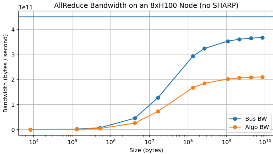
Figure: AllReduce bandwidth on an 8xH100 cluster (intra-node, SHARP disabled).
