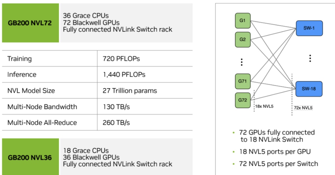
Figure: a diagram showing how a GB200 NVL72 unit is constructed, with 18 switches and 72 GPUs.
