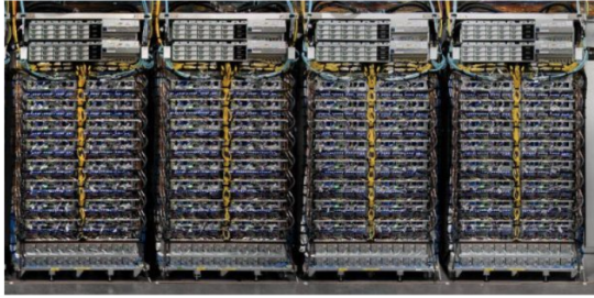
Each rack corresponds to 4x4x4 TPUv4s These can be configured into arbitrary 4x4x4 toruses via optical interconnects
