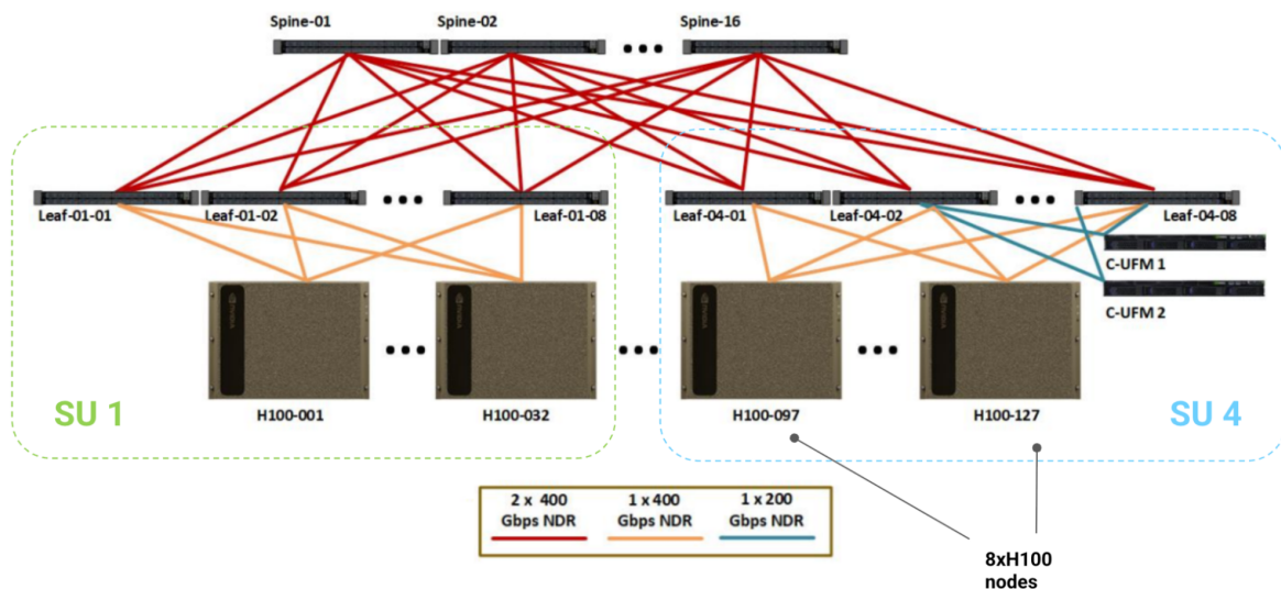
Figure: diagram of the reference 1024 H100 DGX SuperPod with 128 nodes (sometimes 127), each with 8 H100 GPUs, connected to an InfiniBand scale-out network. Sets of 32 nodes (256 GPUs) are called 'Scalable Units' or SUs. The leaf and spine IB switches provide enough bandwidth for full bisection bandwidth between nodes.
