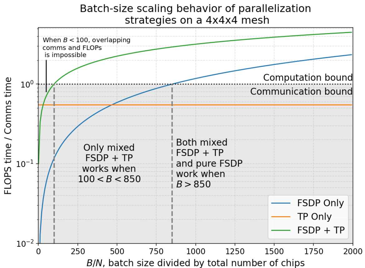
Figure: ratio of FLOPs to comms time for optimal mixed FSDP/TP on a TPUv5p 4 \times 4 \times 4 slice with F=30k . As expected, tensor parallelism has a fixed ratio with batch size; ideal mixed FSDP + TP scales with B , and FSDP scales with B . However, in intermediate batch size regimes, only FSDP + TP achieves a ratio greater than unity.
