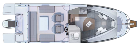
Interior - SUNdeck version
