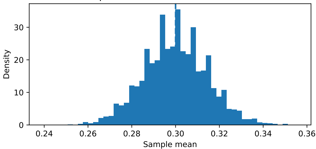
Sample mean distribution for n = 1000
