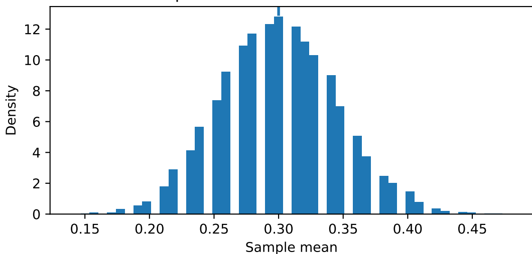
Sample mean distribution for n = 1000
