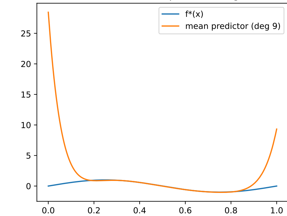
True function vs mean predictor (degree 9)
