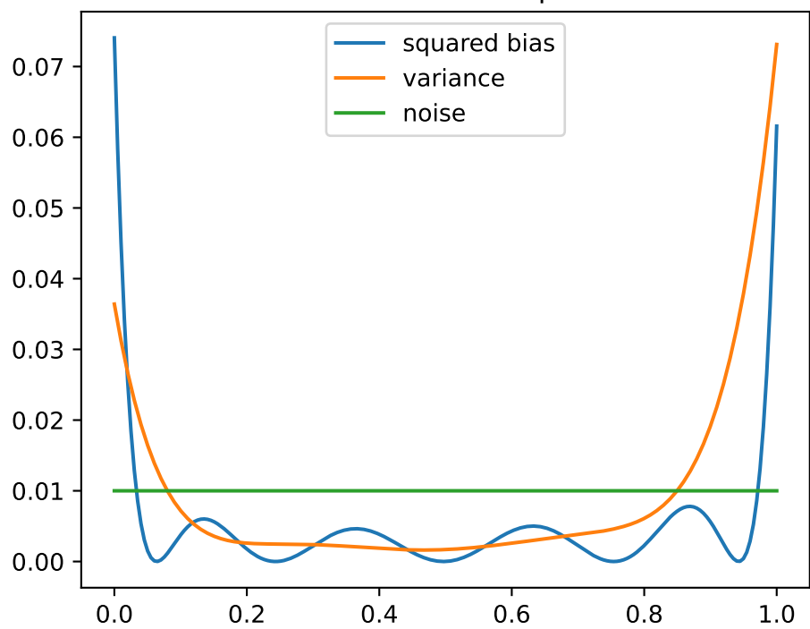
Bias variance decomposition
