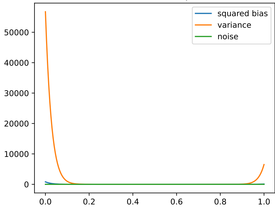
Bias variance decomposition
