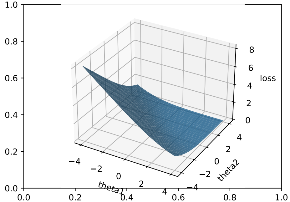
Loss surface
