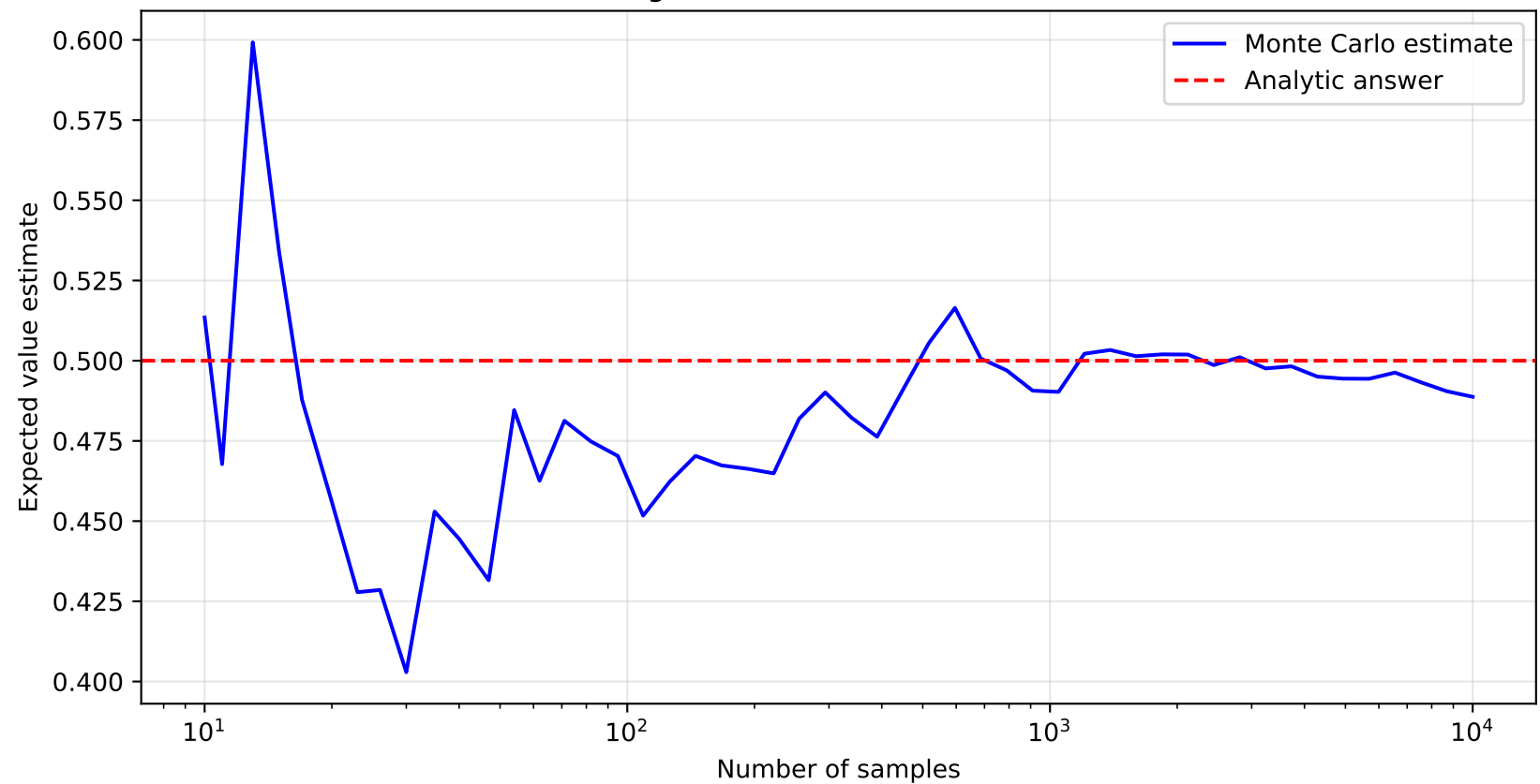
Convergence of Monte Carlo Estimation
