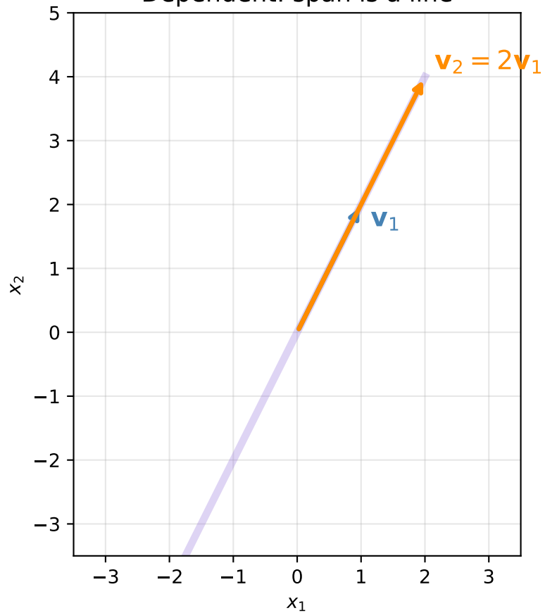
Dependent: span is a line
