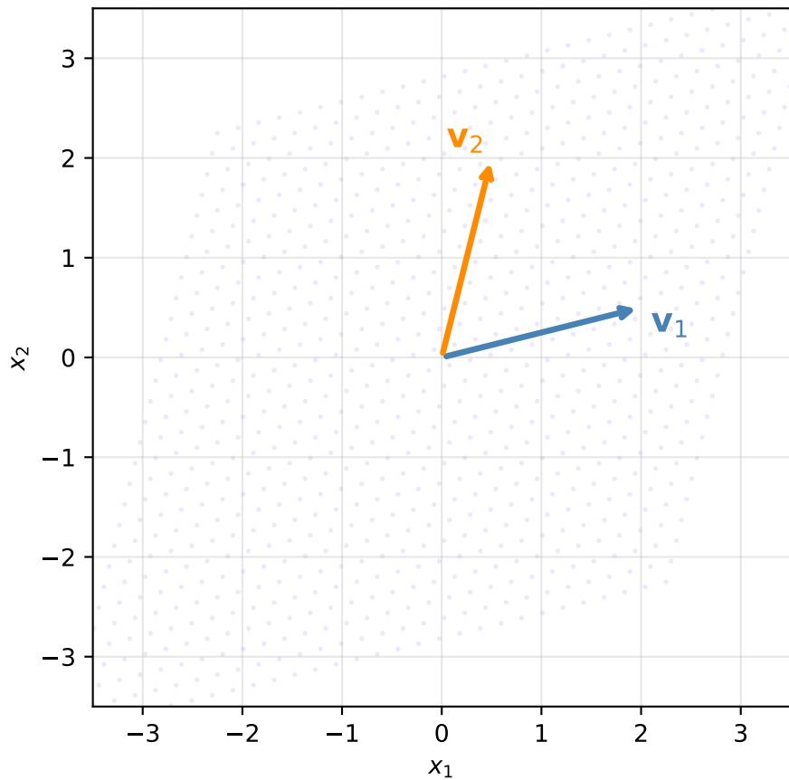
Independent: span is \mathbb{R}^2
