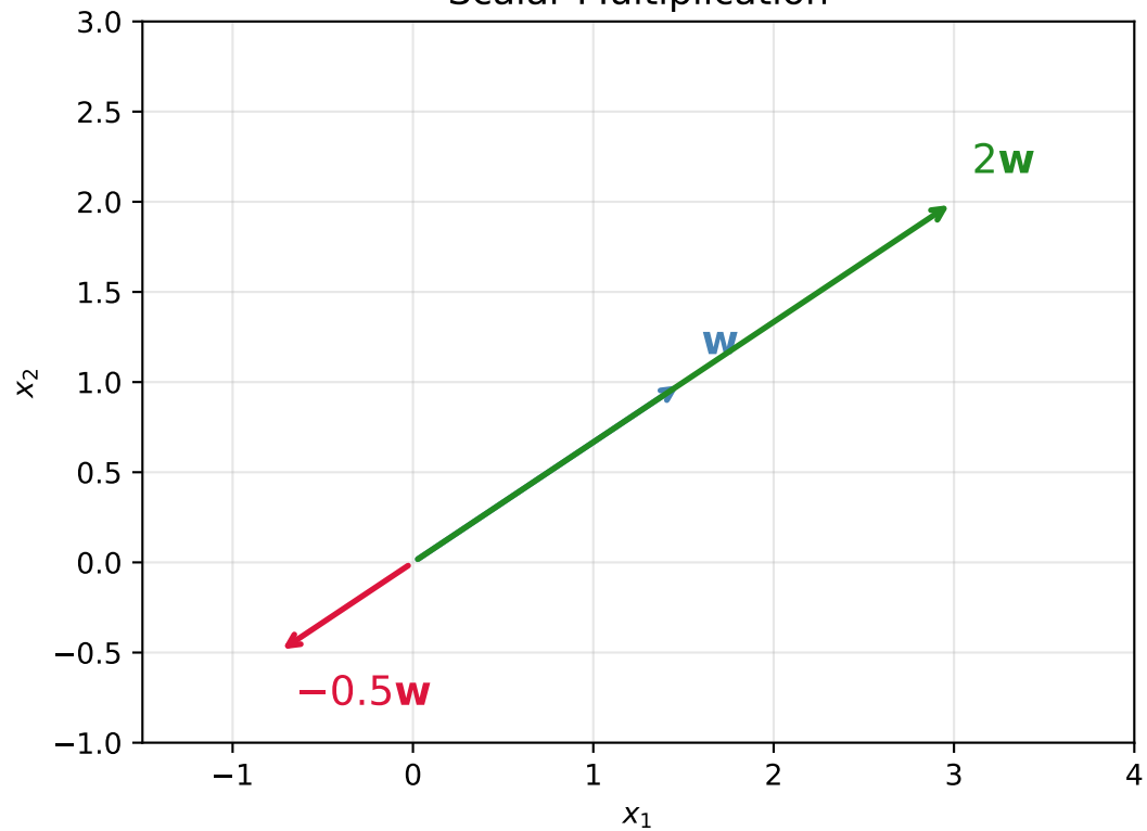
Scalar Multiplication
