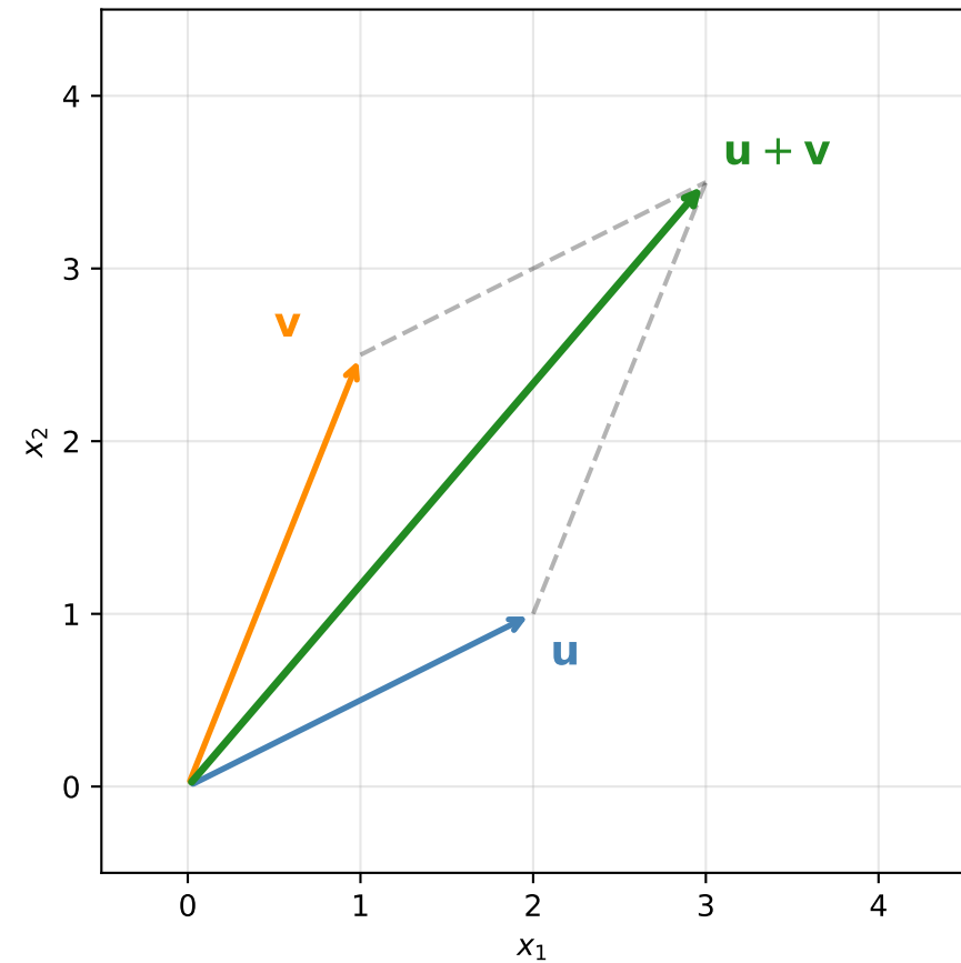
Vector Addition
