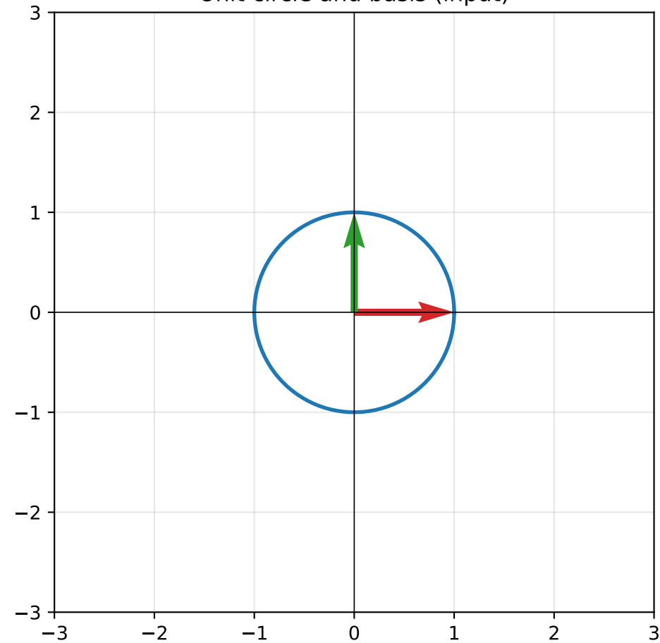
Unit circle and basis (input)
