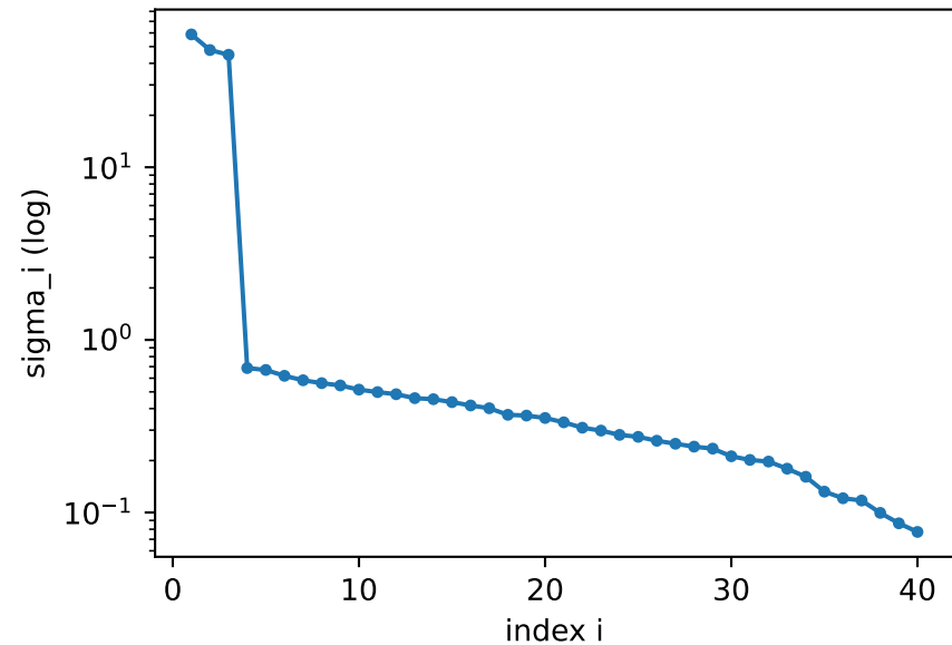
Singular value spectrum
