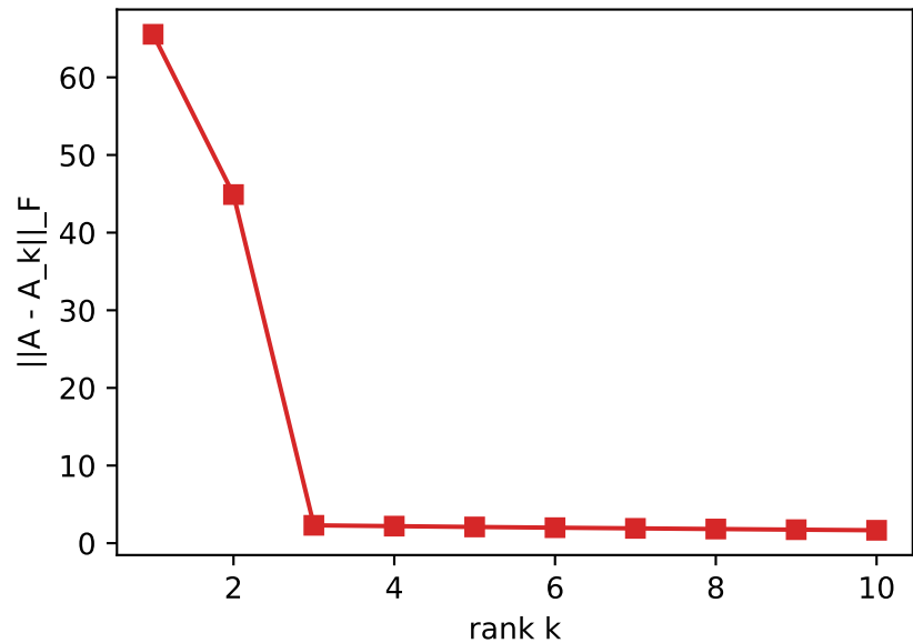
Rank-k Frobenius error
