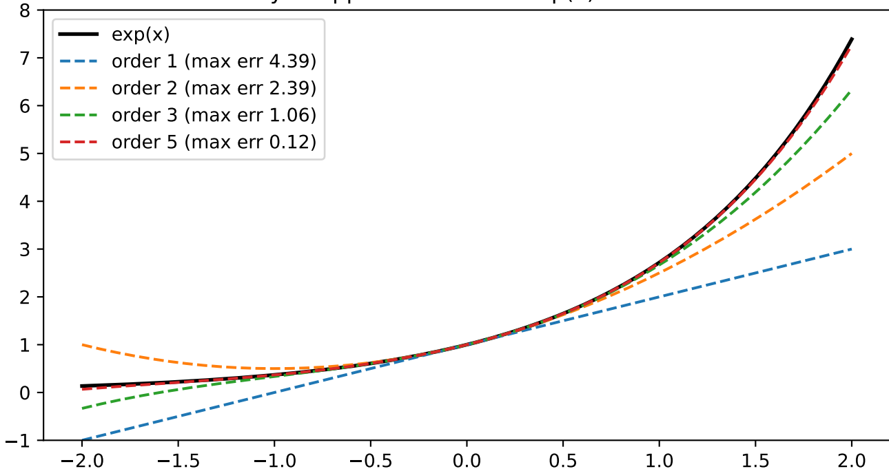
Taylor approximations of \exp(x) about 0
