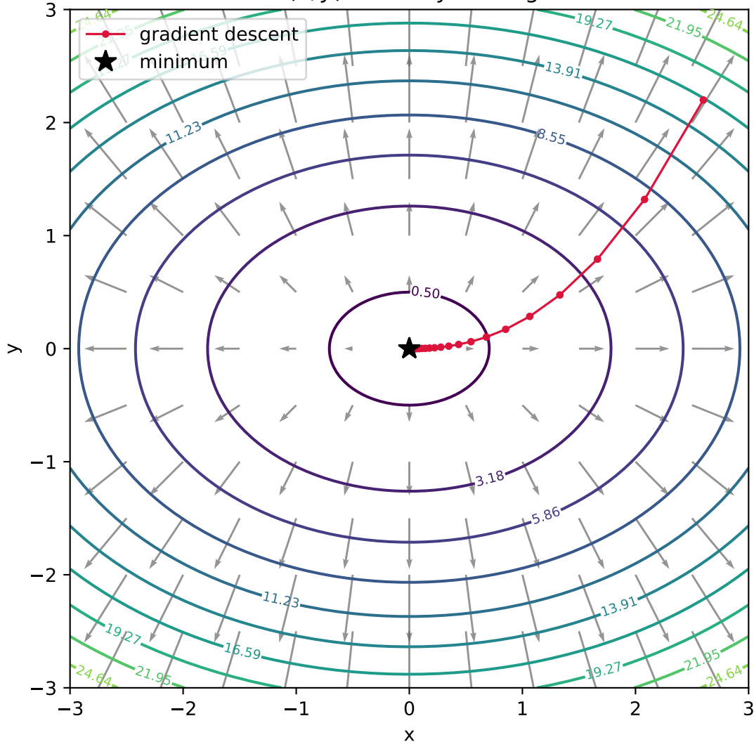
Contours of f(x, y) = x^2 + 2y^2 with gradient field
