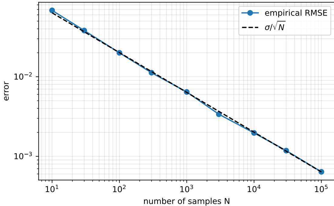
Monte Carlo error decays as 1/\sqrt{N}
