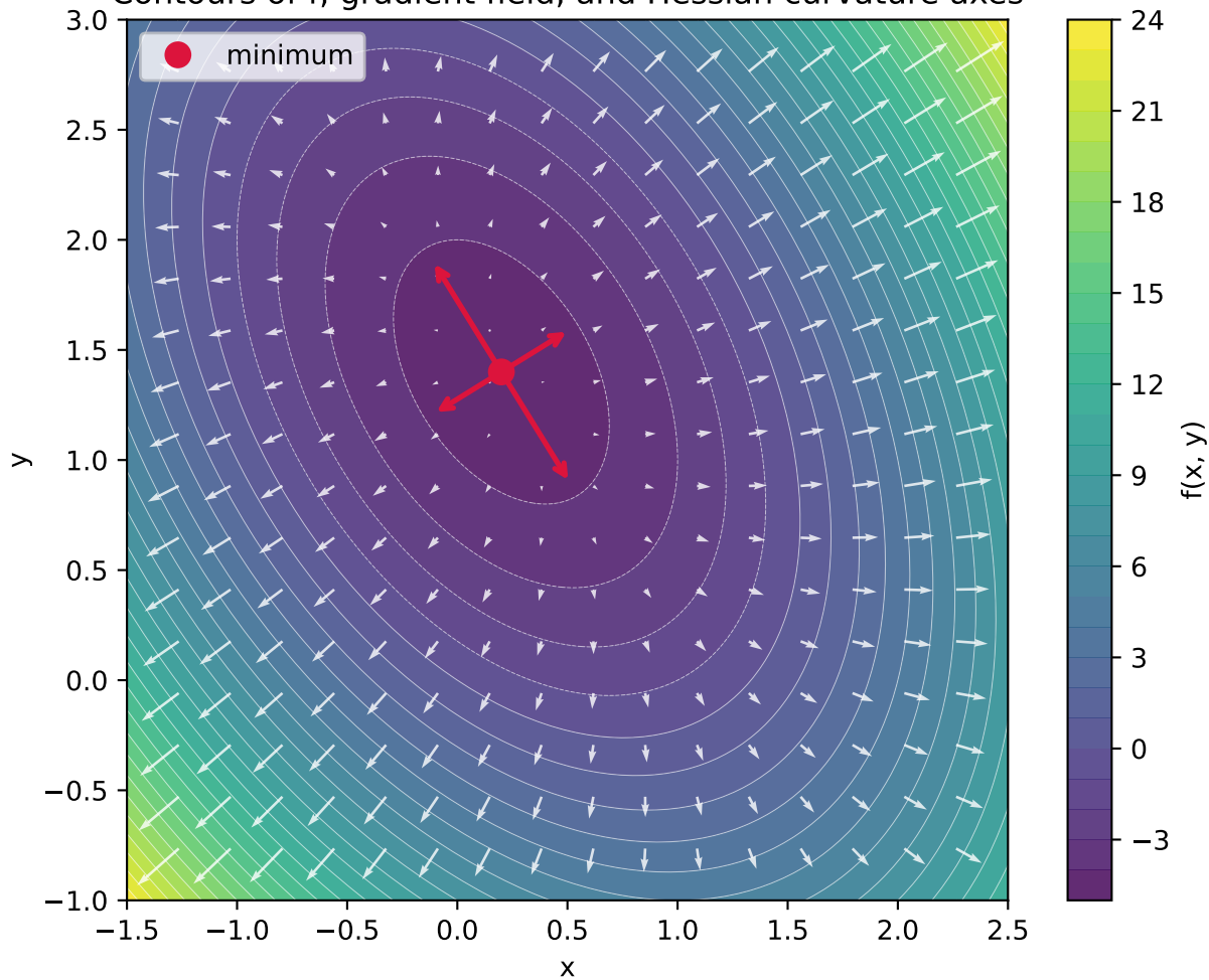
Contours of f , gradient field, and Hessian curvature axes
