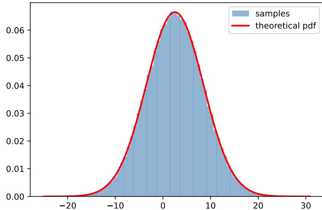
Affine map of a Gaussian
