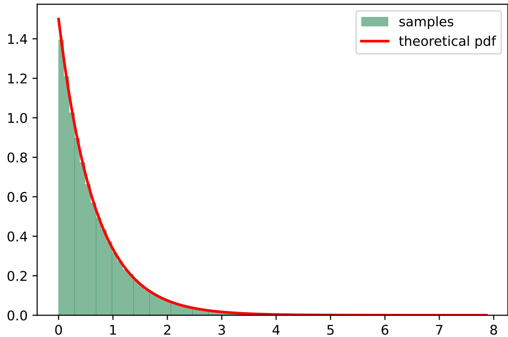
Inverse transform sampling, exponential
