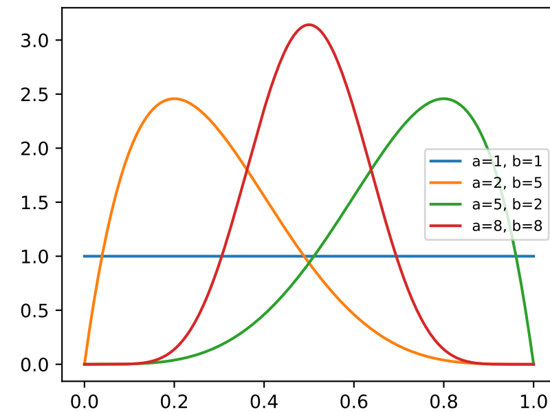
Beta densities
