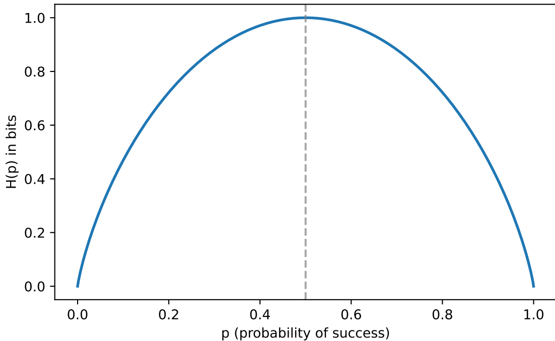
Entropy of a Bernoulli variable
