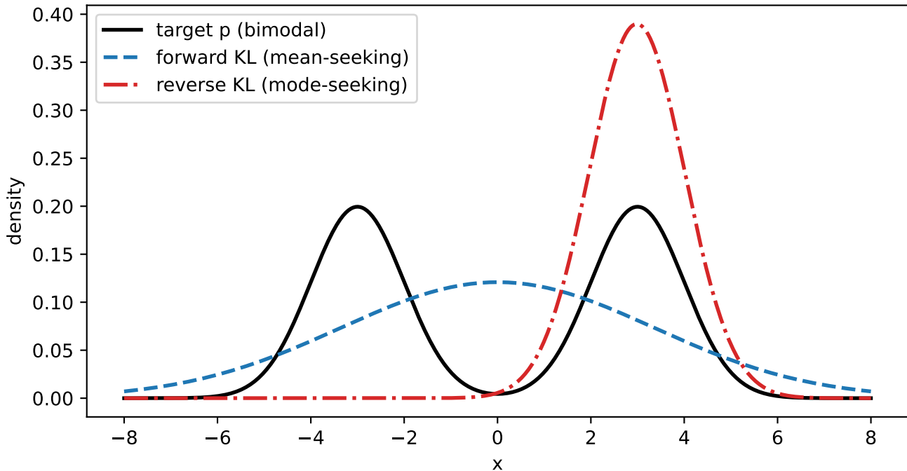
Forward vs reverse KL fit to a bimodal target
