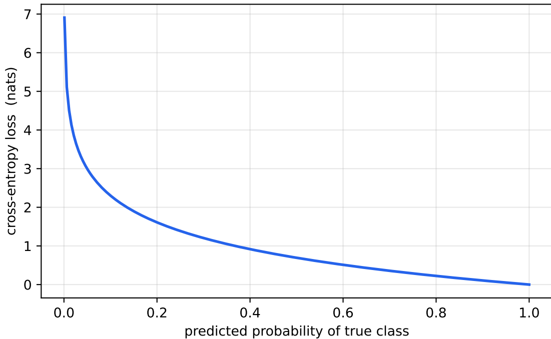
Cross-entropy loss vs predicted probability
