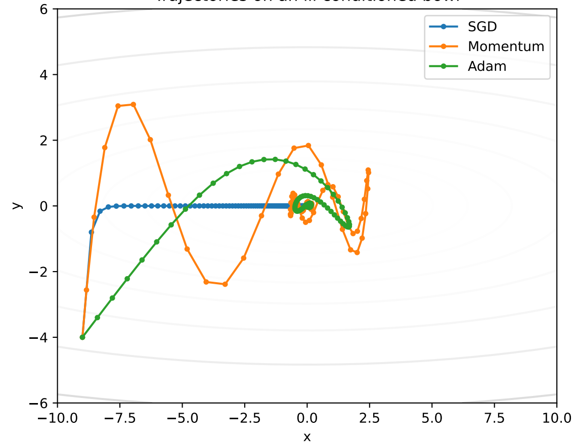
Trajectories on an ill conditioned bowl
