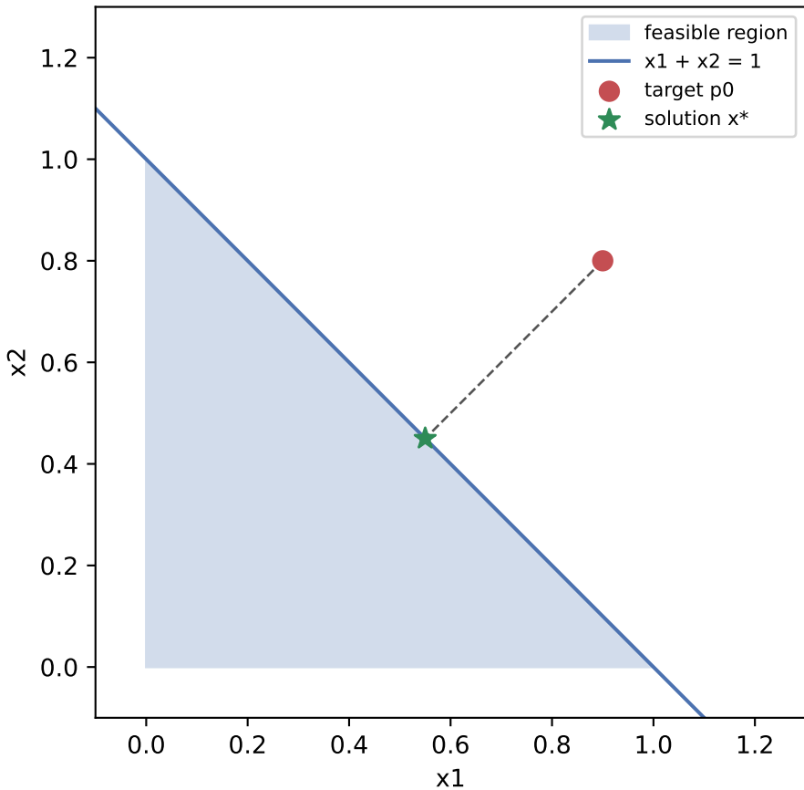
Projection onto a constrained region
