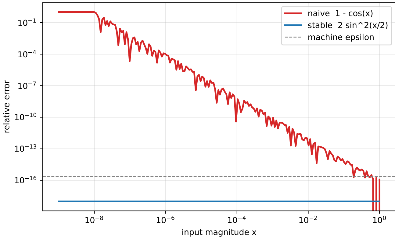
Catastrophic cancellation: naive vs stable 1 - \cos(x)
