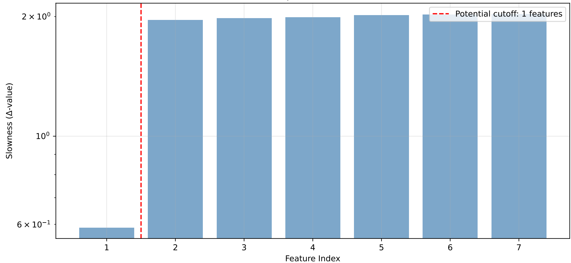
Slowness Spectrum (Credit Data)
