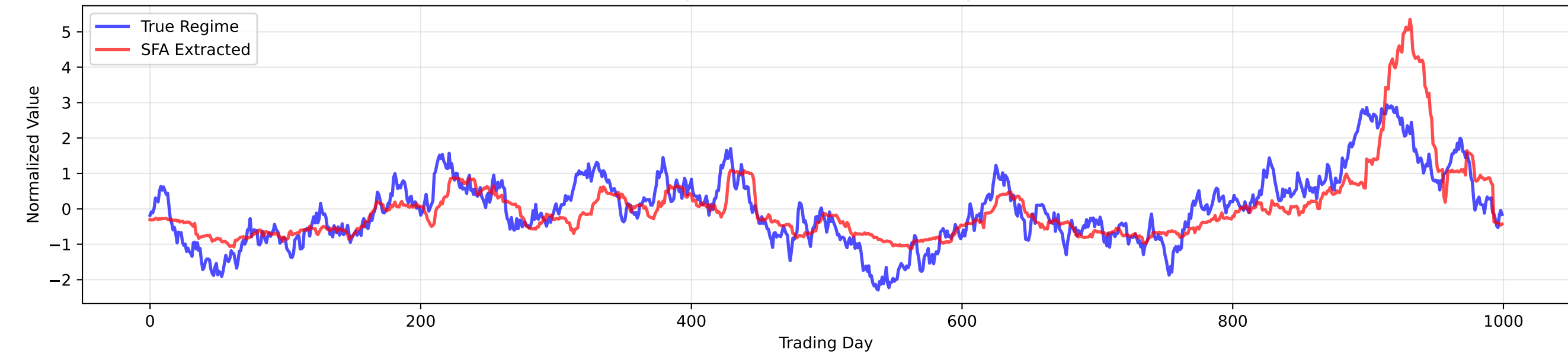
Comparison: True vs Extracted Regime
