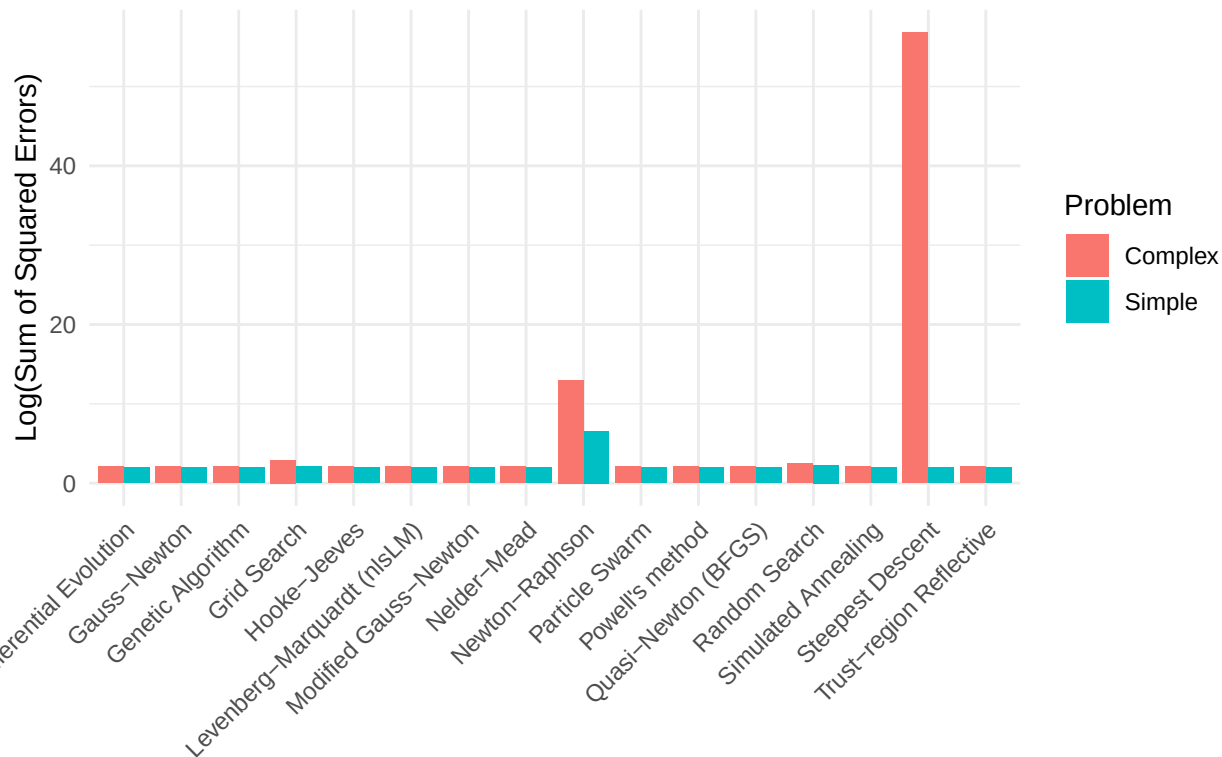
Comparison of SSE by Method and Problem Complexity
