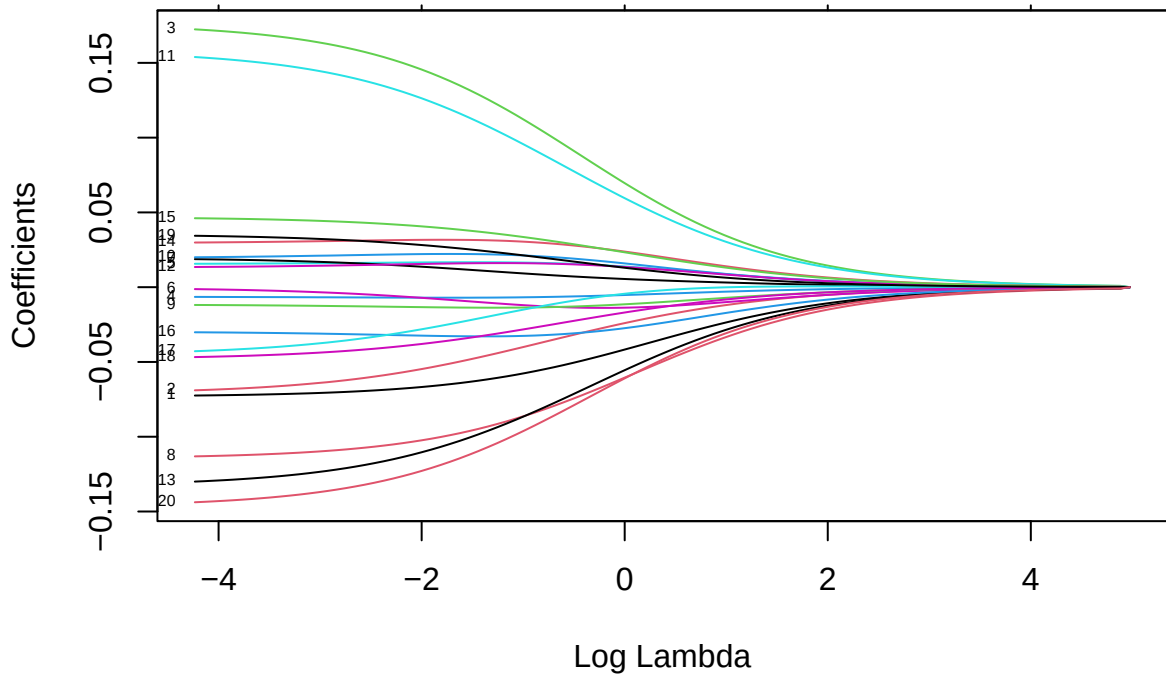
Coefficient Paths for Ridge Regression
