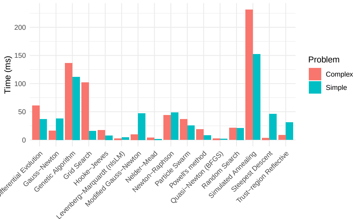
Comparison of Computation Time by Method and Problem Complexity
