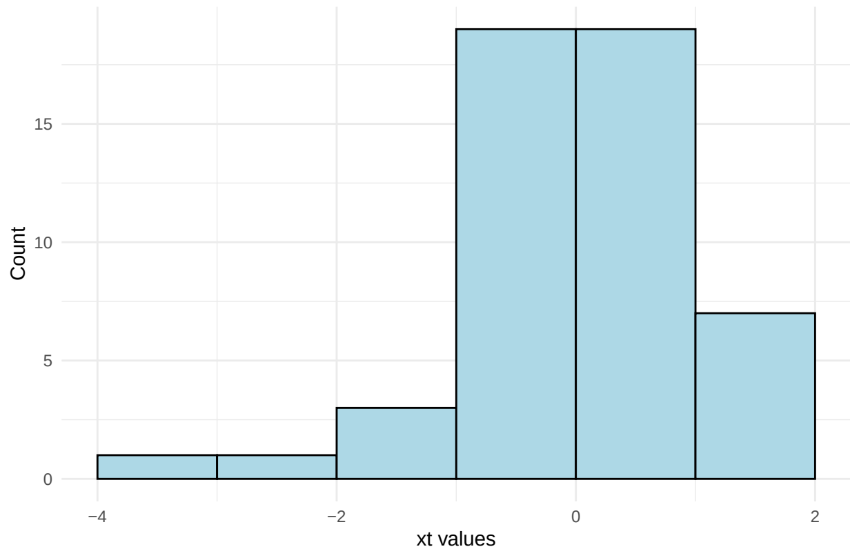
Histogram of x_t
