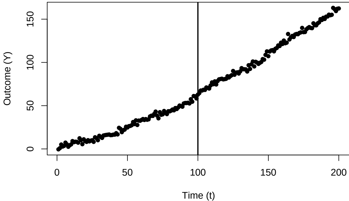
Full Time Series with True Jump at T_{\text{star}}
